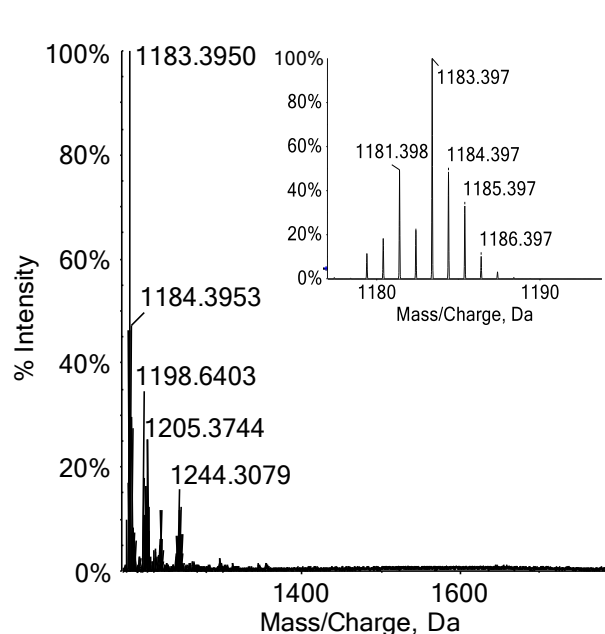
Figure 5 ESI-MS spectrum of the C-terminal dodecapeptide hTrxR (Ac-SGGDILQSGCUG-NH 2 ) dissolved in MilliQ water (10 -4 M). The inset shows the characteristic selenium isotopic pattern.
