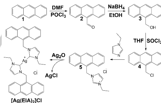
Scheme 1 Synthetic route for bis(1-(anthracen-9-ylmethyl)-3-ethylimidazol-2-ylidene) silver chloride.
