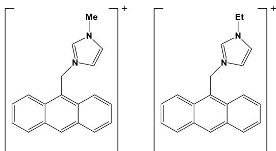
Figure 1 Structures of the ligand previously reported (left) 7 and of the modified ligand used in this work (right, (5) in Scheme 1).
