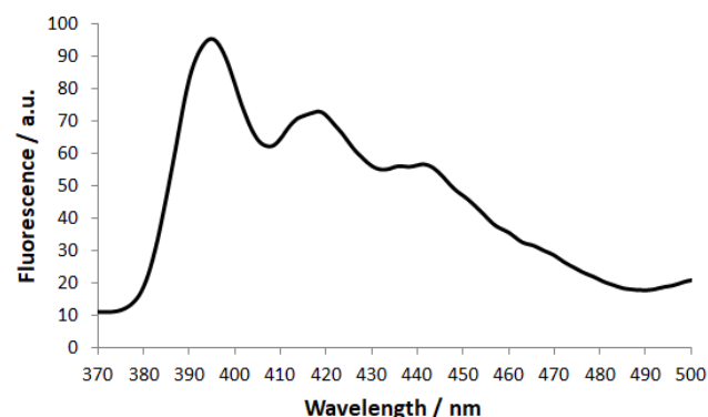
Figure 4 Emission spectra of [Ag(EIA) 2 ]Cl (10 -8 M in 50 mM phosphate buffer pH 7.4 in presence of 0.001% DMSO) \lambda_{exc}=350 nm.
