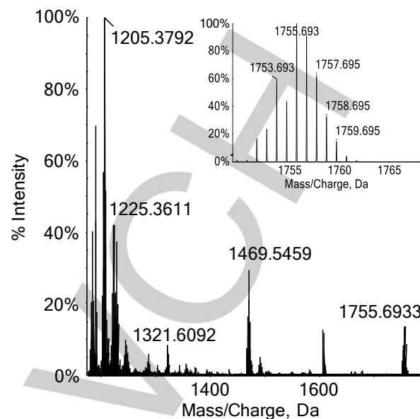
Figure 6 ESI-MS spectrum of the C-terminal dodecapeptide hTrxR (Ac-SGGDILQSGCUG-NH 2 ) dissolved in MilliQ water (10 -4 M) in presence of 5.0 eq. of dithiothreitol (DTT) and 1.0 eq. of [Ag(EIA) 2 ]Cl incubated for 2 h at 37 °C. The inset shows the isotopic pattern for the bis-adduct.
