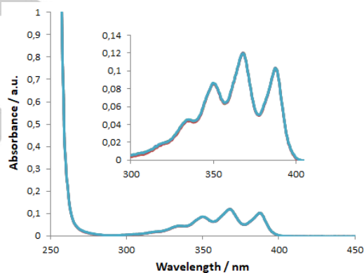
Figure 3 Time course spectra of [\text{Ag}(\text{EIA})_2]\text{Cl} ( 10^{-5} M, phosphate buffer 50 mM pH 7.4, 1% DMSO) for 24 h; see supporting material for UV-Vis spectrum in pure DMSO and DMF.
