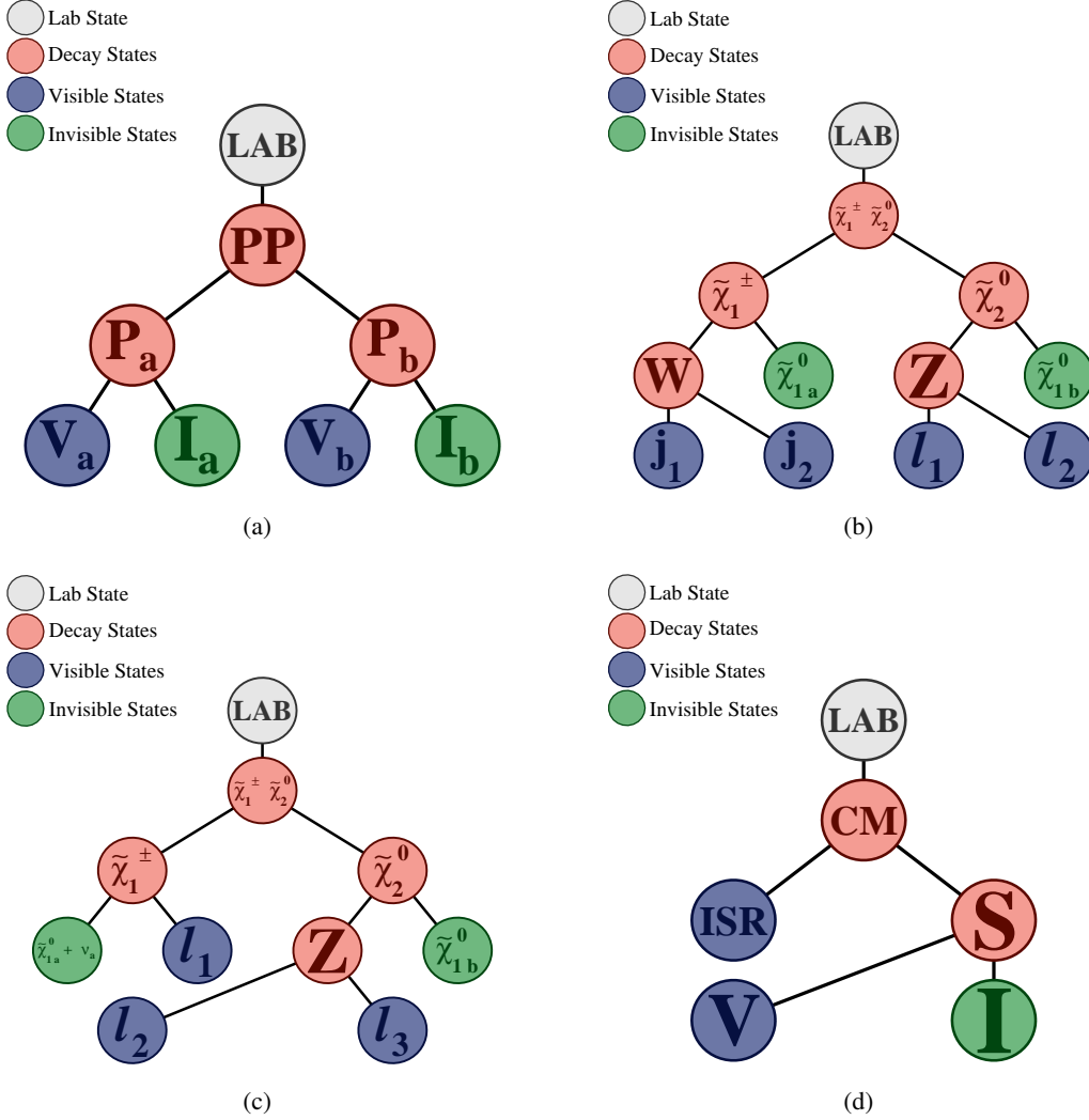
Figure 2: (a) The “standard” decay tree applied to pair-produced sparticles (“parent” objects), P, decaying to visible states “V” and invisible states “I”. (b) Decay trees for the 2\ell + 2 jets final state and (c) 3\ell final state. (d) The “compressed” decay tree. A signal sparticle system S decaying to a set of visible momenta V and invisible momentum I recoils from a jet-radiation system ISR.
