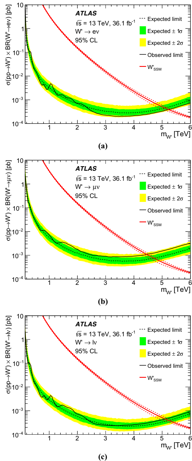
Fig. 2 Observed (solid black line) and expected (dashed black line) upper limits on cross-section times branching ratio ( \sigma \times BR ) as a function of the SSM W' boson mass in the a electron, b muon and c combined electron and muon channels. The 1\sigma (green) and 2\sigma (yellow) expected limit bands are also shown. The predicted \sigma \times BR for SSM W' production is shown as a red solid line. For illustration the uncertainties in \sigma \times BR from the PDF, \alpha_s and the renormalisation and factorisation scales are also shown as red-dashed lines
