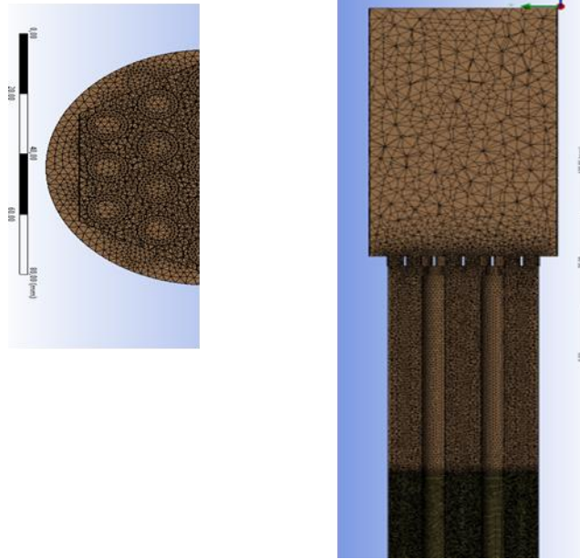
Figure 6 Computational mesh C adopted for the simulations
