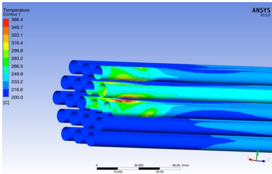
Figure 9 Clad temperature field in the region behind the blockage (blockage type 1).
