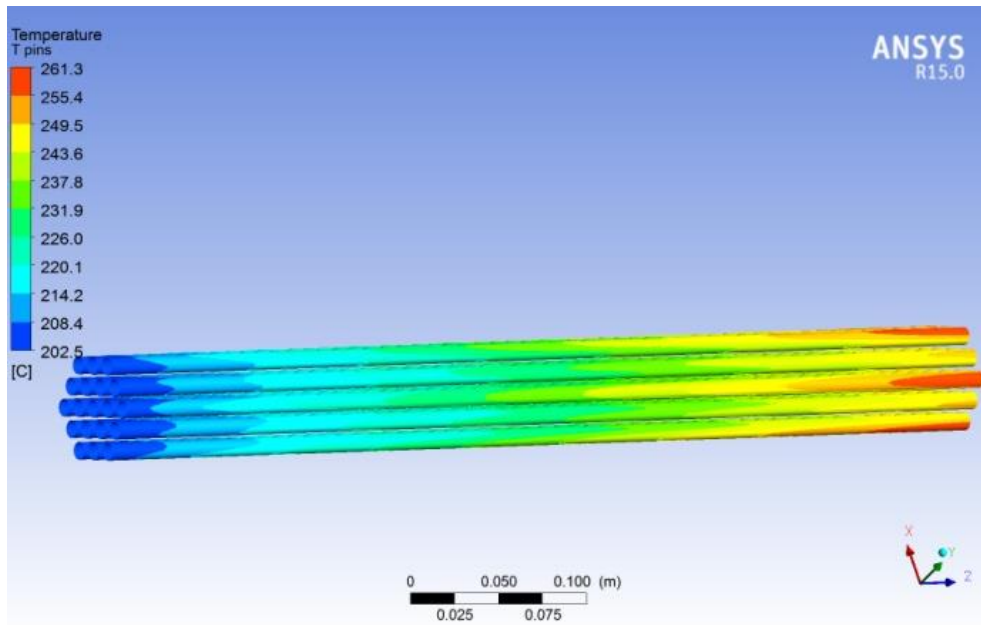
Figure 8 Pin clad temperature field in the unblocked case.
