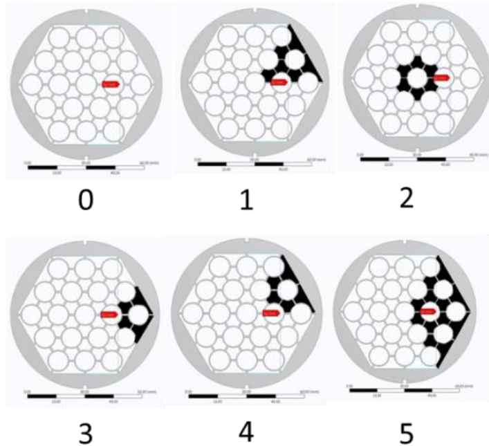
Figure 7 Different blockage types: (0) unblocked; (1) sector; (2) central; (3) corner; (4) edge; (5) two sectors. Subchannels are blocked with a stainless steel caps fixed to the grid spacer (in gray).
