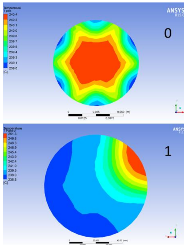
Figure 11 Temperature distribution in the outlet section of the mixing region for case 0 (unblocked) and 1 (sector blockage).
