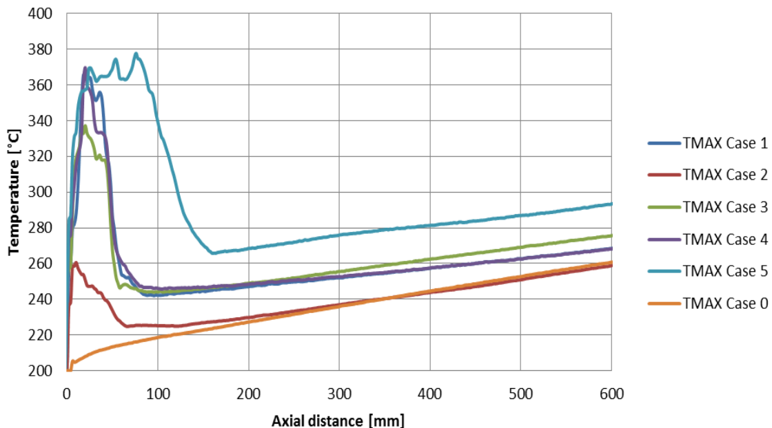
Figure 12 Maximum temperature profile along the streamwise axial direction for the 6 cases investigated.
