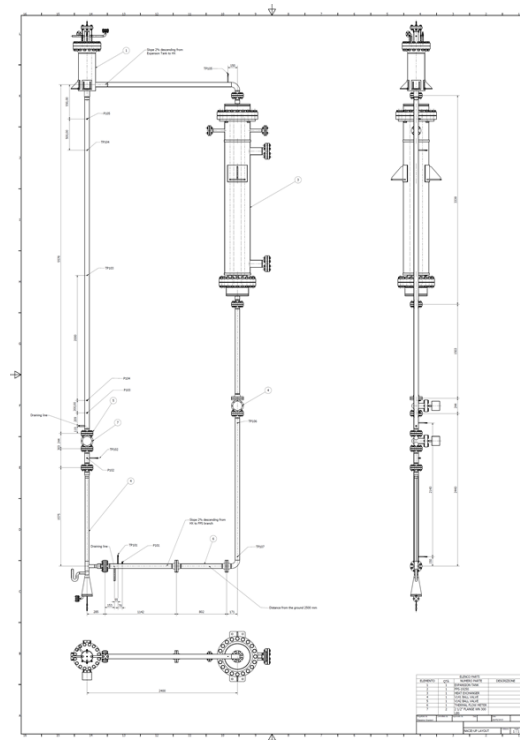
Figure 1 Technical drawing and main dimension of the NACIE-UP loop.
