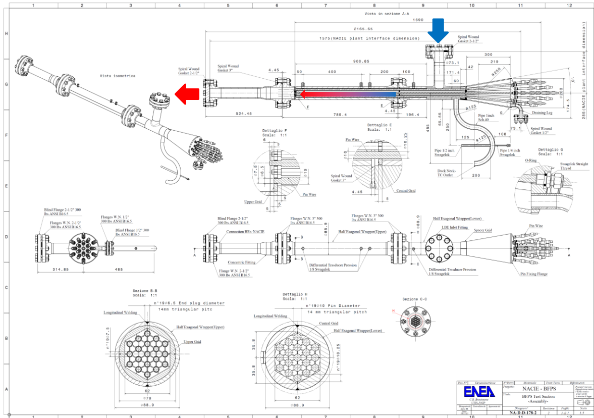
Figure 2 Mechanical drawing of the BFPS test section.
