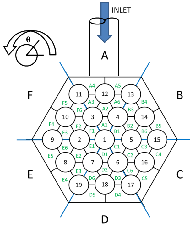
Figure 13 Sketch of a section of the new fuel pin bundle simulator for the NACIE-UP facility as viewed from the top.
