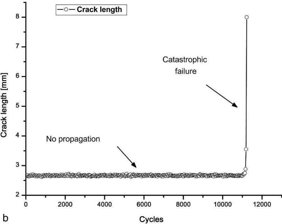
Fig. 5 – Comparison of crack propagation behavior for SBR (a) and BR (b) compound with SENT geometry.
