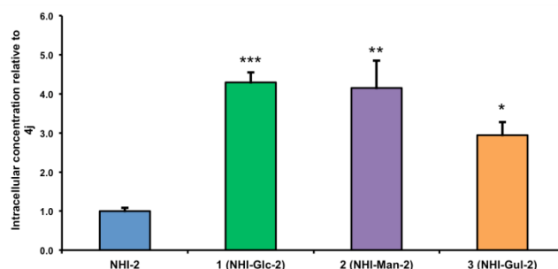
Fig. 4 Results of the intracellular concentration comparison study comparing relative uptake of NHI-2 ( 15 ) to its three glycoconjugates 1-3 . A549 non-small cell lung carcinoma cells were treated with 100 \mu\text{M} concentrations of each compound for 4 hours; cells were then lysed, sonicated in methanol, and assessed for intracellular compound concentration by LC-MS. Triplicate data is shown, with error bars denoting standard error. Statistical analysis was performed using an unpaired Student's t test to compare glycoconjugate intracellular concentrations with NHI-2 intracellular concentration, with * denoting p < 0.05 , ** denoting p < 0.01 , and *** denoting p < 0.0005 .
