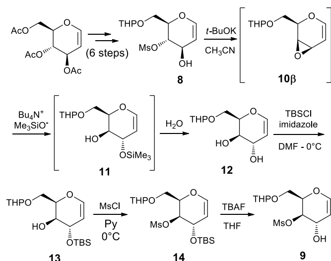
Scheme 2 Synthesis of THP-protected trans -hydroxymesylates 8 and 9 from tri- O -acetyl- D -glucal.
