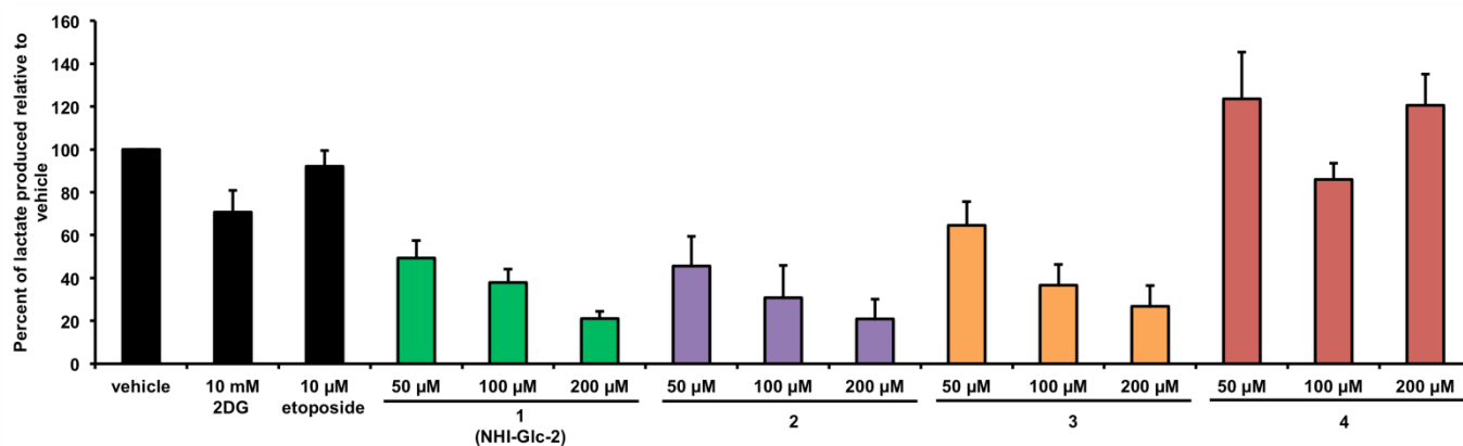
Fig. 3 Lactate production inhibition of glycoconjugates 1-4 . HeLa human cervical carcinoma cells were treated under normoxic conditions with indicated compound concentrations or 1% DMSO vehicle, in DMEM supplemented with 10 mM unlabeled glucose, 1 mM pyruvate, and 4 mM glutamine. Following 8 hour incubation, medium aliquots were collected, concentrated, derivatized using MTBSTFA + 1% TBDMCS catalyst, and assessed by GC-MS. Lactate was normalized in each sample using the 1 mM chlorophenylalanine (CPA) internal standard, and lactate relative to vehicle is depicted. Averages from three or more independent experiments are depicted, with error bars depicting standard error ( n \geq 3 ).
