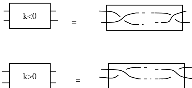
FIGURE 6. The boxes used in Figure 5.
