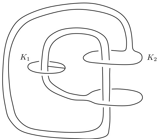
FIGURE 24. The spine of a (4)_L -unknotted handlebody which is (3)_L -knotted.
