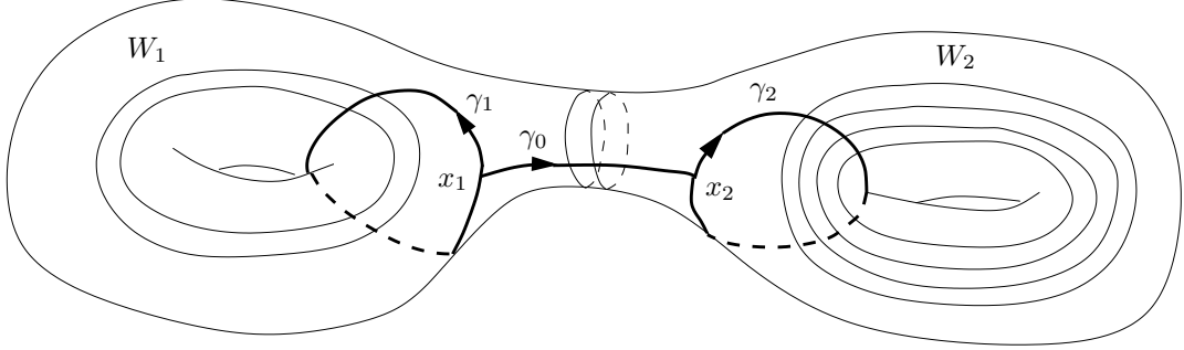
FIGURE 22. The definition of handlebody pattern.
