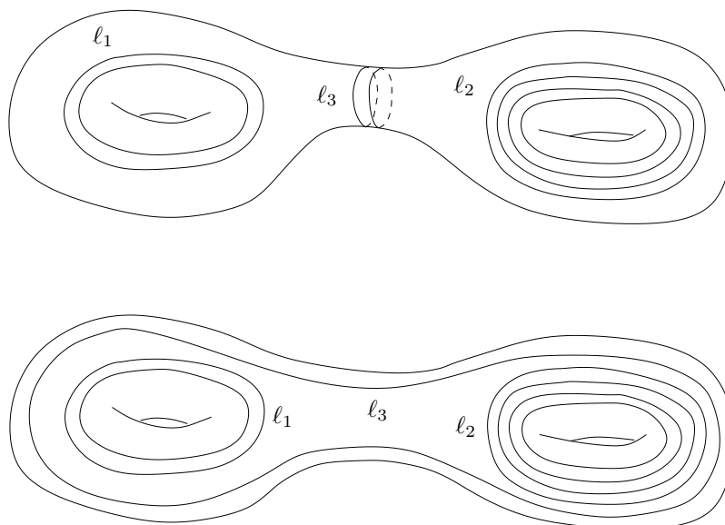
FIGURE 21. The boundary components of a cut system \mathcal{S} . On the top: l_3 separates \partial M , so \mathcal{S} is good. On the bottom: l_3 does not separate \partial M , and \mathcal{S} is not good.
