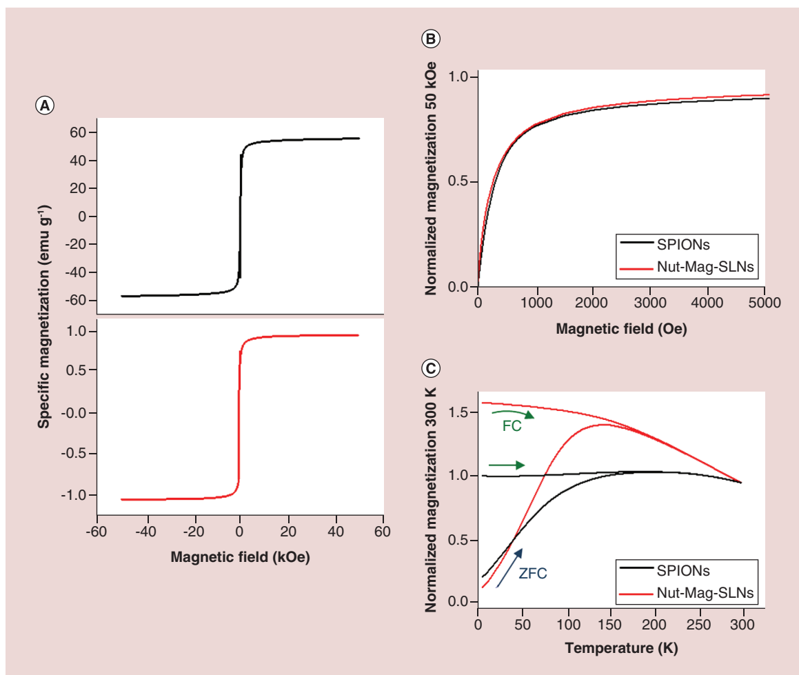
Figure 2. Magnetic characterization of nutlin-loaded magnetic solid lipid nanoparticles. (A) Hysteresis loops of the bare SPIONs (top) and of the Mag-SLNs (bottom) measured at room temperature. (B) Normalized magnetization as function of the field in the low field region of the bare SPIONs and of the Nut-Mag-SLNs. The normalization was done with the respect to the magnetization measured at 50 kOe. (C) Temperature dependence of the normalized magnetization of the bare SPIONs and of the Nut-Mag-SLNs using the ZFC and FC procedures. The normalization was performed at the magnetization value at room temperature.
