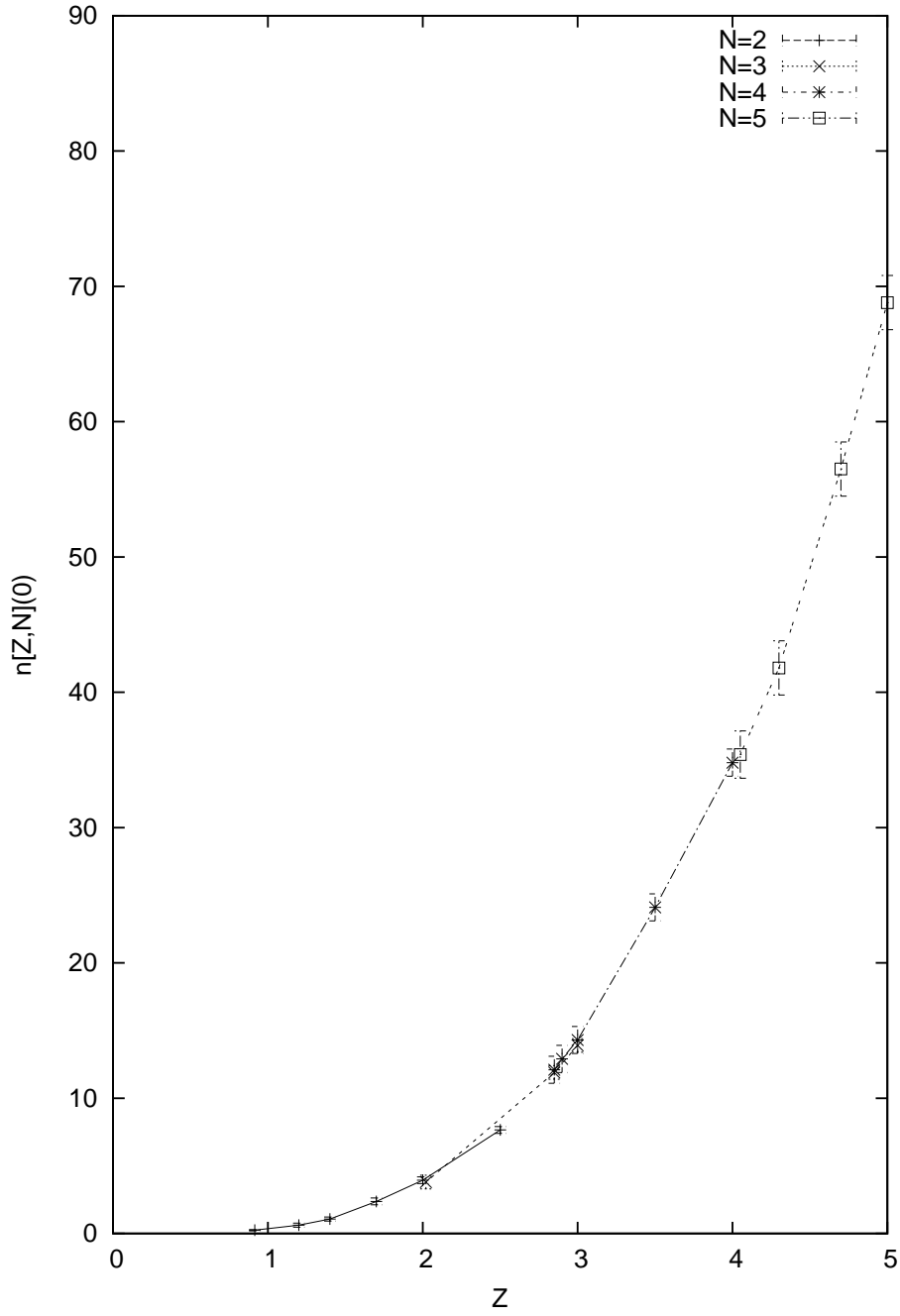
Figure 1: Plot of the electron density at the nucleus n_0[Z, N] as a function of the fractional nuclear charge Z for the four series of atomic ions considered in this work. Neutral atoms correspond to the case N = Z . These are the only observables.
