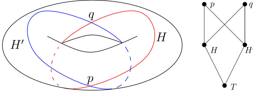
FIGURE 1. The toric arrangement of Example 2.3.6 and its poset.
