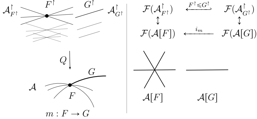
FIGURE 2. A pictorial representation of the notations introduced here. The “abstract” arrangements \mathcal{A}[F] serve as a model for the localizations \mathcal{A}_{F^\dagger}^\dagger , and the map i_m is induced at the abstract level by the inclusion defined by a(ny) lift of the morphism m to \mathcal{F}(\mathcal{A}^\dagger) .
