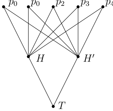
FIGURE 3. The poset of layers associated to the arrangements \mathcal{A}^1 and \mathcal{A}^2 of Example 7.3.2.
