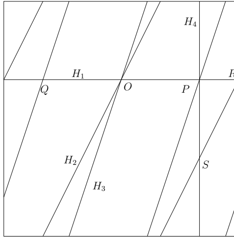
FIGURE 4. Example of a toric arrangement with cohomology ring not generated in degree 1.
