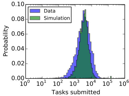
Fig. 9 Distribution of number of submitted tasks for the synthetic workload ( Simulation ), compared to the real workload ( Data ). The synthetic workload shows less variation than the real workload.
