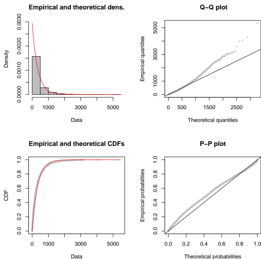
Fig. 6 Machine update inter-event times, fitted with an exponential distribution. The left panels show the density and cumulative distribution functions, with the lines representing exponential fitting and the bars/circles showing real data. The right panels show goodness of fit in Q-Q and P-P plots (straight lines show perfect fit).
