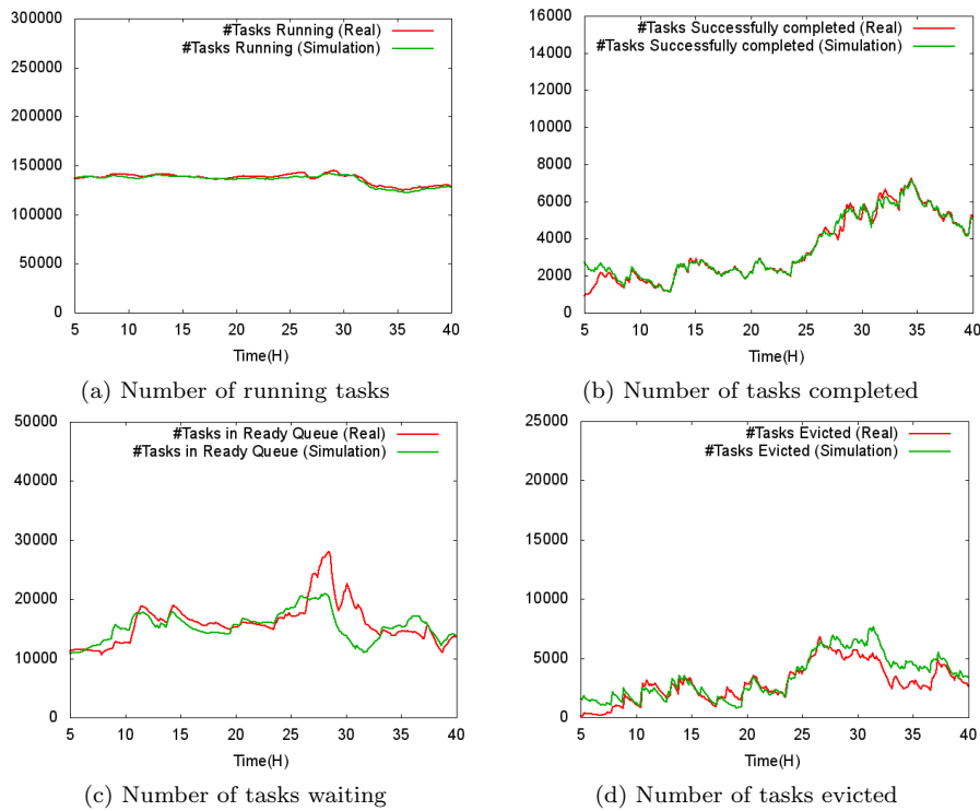
Fig. 10 Simulation and real data for four different metrics. All show good agreement between the behavior of our model and that of the real system.
