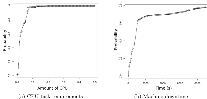
Fig. 7 Examples of CDFs fitted by sequences of splines, obtained with BiDAL. The circles represent the data, while the lines show the fitted splines. The CDFs are employed to produce synthetic traces to be used as input to our model.
