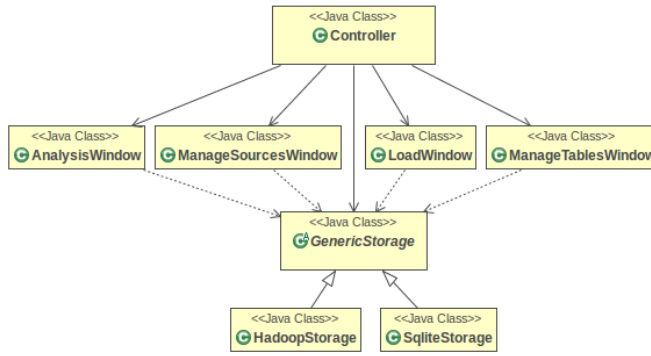
Fig. 2 UML diagram of BiDAI classes. This shows the modular structure where the storage is separated from the user interface, facilitating addition of new types of storage backends.
