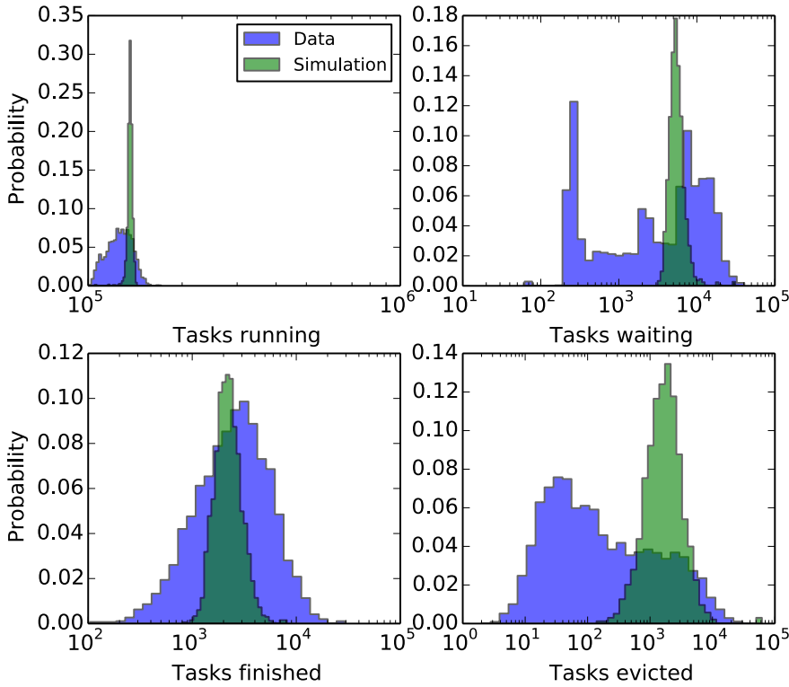
Fig. 8 Distribution of number of tasks in different categories for each 450s time window, for the synthetic-trace-driven simulation compared to the real data . The y-axis shows the fraction of time windows with the corresponding number of tasks running, waiting, finished or evicted. Average behavior is similar between simulation and data for all categories except tasks evicted. However, variability is larger in the data for all cases.
