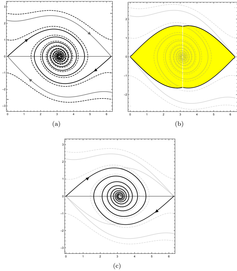
FIGURE 1. The dissipative pendulum with \lambda = 1/5 . (a): Phase portrait where we highlight the stable and unstable manifolds of the saddle (thick gray and thick black respectively). (b) The sets \mathcal{Z}_{F_\lambda}^0 (thick black line) and \mathcal{Z}_{F_\lambda}^- (shaded region). (c) The global maximal attractor formed by the unstable manifolds and the equilibria.
