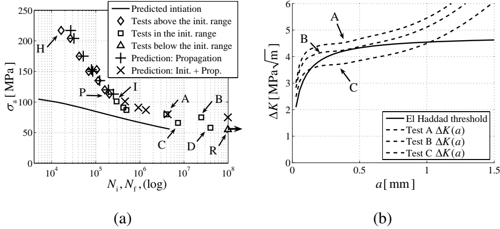
Fig. 9. Notched geometry results: (a) prediction fatigue life compared with the experimental results, (b) non propagating crack prediction.
