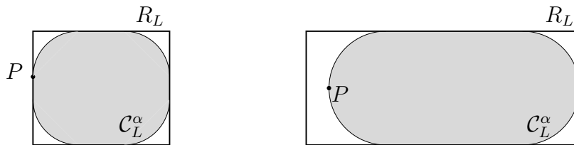
FIGURE 1. The two possible shapes of the \alpha -Cheeger sets in rectangles.
