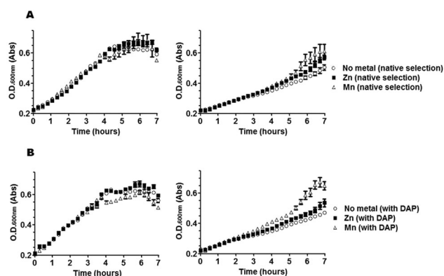
Fig. 3 Effect of metal supplementation on growth curves of bacterial cultures selected for DapE activity (A) or non-selected (B), in the absence of L-captopril (left) or in the presence of 25 mM L-captopril (right). Cultures were grown in LB broth either in the presence or absence of mDAP for selection of native (desuccinylase) activity of DapE. The effect of divalent Zn or Mn was tested and compared to the absence of metal supplementation (no metal). Note that L-captopril toxicity is dependent on metal-supplementation and that \text{Mn}^{2+} is more protective than \text{Zn}^{2+} , although the toxic effect of the drug is largely independent of DapE activity. Means of measurements from quadruplicate cultures are plotted with standard deviations shown as error bars.
