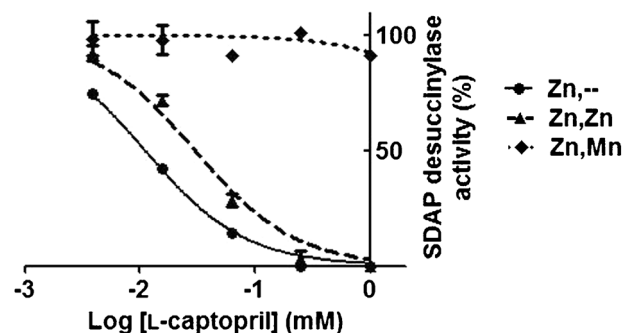
Fig. 1 Inhibition of desuccinylase activity of different DapE metallo-isoforms by L-captopril. Measurements were carried out in triplicate and error bars represent the standard deviation from the mean.
