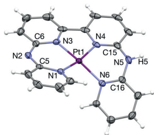
Figure 1. Displacement ellipsoid plot (50% probability level) of the cationic moiety [Pt(Hbabppy)] + as observed in the crystal structure of [Pt(Hbabppy)]PF 6 . Counteranions have been omitted for clarity. [21]
