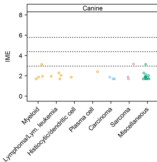
FIGURE 6 Integrated metric of evidence (IME) values for cancer types in dogs. Horizontal dotted lines indicate the threshold IME values between negligible and low (2.95), low and intermediate (4.37), and intermediate and high (5.78) levels of evidence. Miscellaneous cancer types included pheochromocytoma, unspecified abdominal, adrenal, bladder, cardiac, mediastinal, and splenic masses, other hematopoietic tumors, and unspecified neoplasia. Lym., lymphoid; Myeloid, myeloid leukemia or myeloproliferative disease
