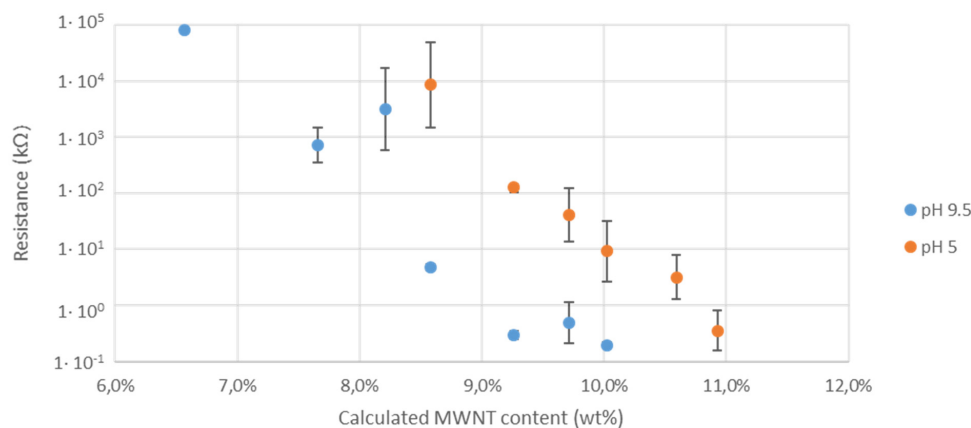
Figure 9. The electrical resistance of composites made from PS 26 PAA 580 polymer. Increasing the wt% of MWCNTs results in reduced resistance. For every sample an acidic (pH 5) and alkaline (pH 9.5) composite was made.
