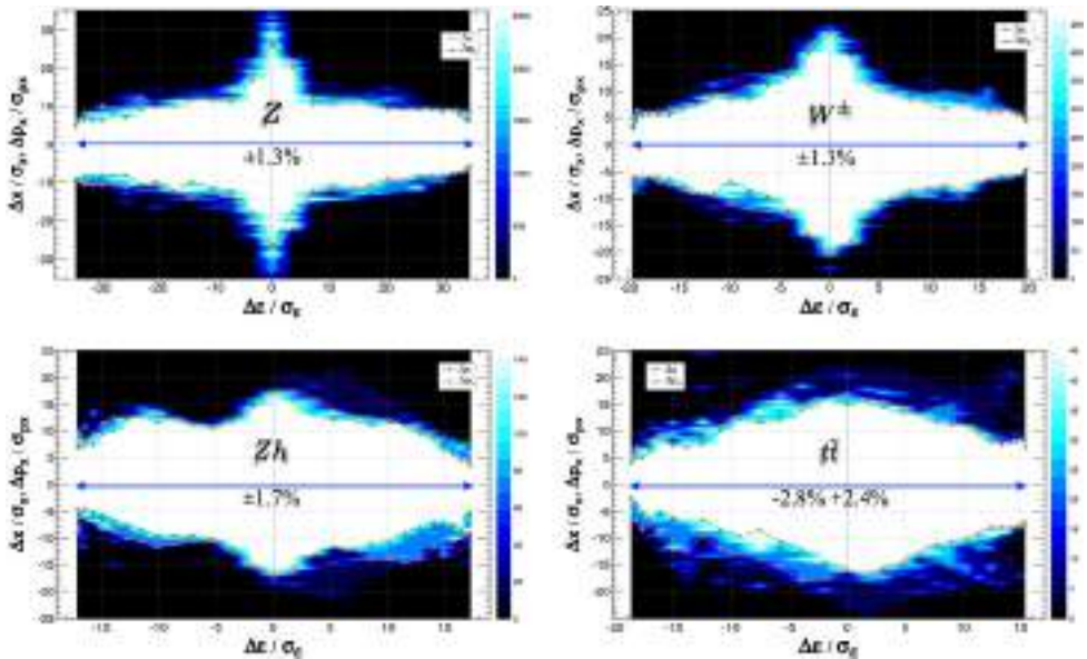
Fig. 2.11. Dynamic apertures in z-x plane after sextupole optimisation with particle tracking for each energy. The initial vertical amplitude for the tracking is always set to J_y/J_x = \varepsilon_y/\varepsilon_x . The number of turns corresponds to about 2 longitudinal damping times. The resulting momentum acceptances are consistent with the luminosity optimisation shown in Table 2.1. Effects in Table 2.3 are taken into account. The momentum acceptance at \bar{t}\bar{t} is “asymmetric” to match the distribution with beamstrahlung.
