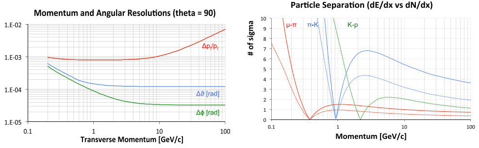
Fig. 7.10. IDEA drift chamber performance. Left: momentum and angular resolutions for \theta = 90^\circ as a function of momentum. Right: particle type separation in units of standard deviations as a function of momentum, with cluster counting (solid curves) and with dE/dx (dashed curves).
