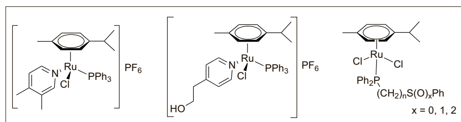
Fig. 5. Ru(II) p -cymene complexes with pyridine ligands or chelating P,S ligands.
