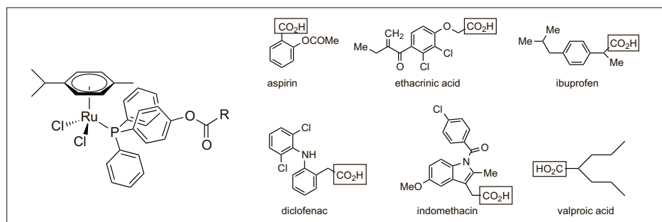
Fig. 9. Functionalization of p -cymene complexes with bioactive carboxylic acids (RCO 2 H), obtained by direct esterification of coordinated (4-hydroxyphenyl)diphenylphosphine.
