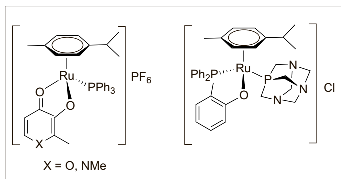
Fig. 6. Cationic Ru(II) arene complexes with mono- or bidentate triphenylphosphine ligands.
