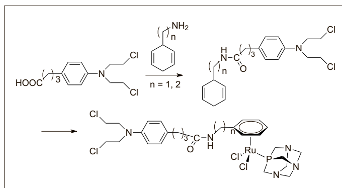
Scheme 3. Synthesis of chloroambucil-functionalized arene RAPTA complex.
