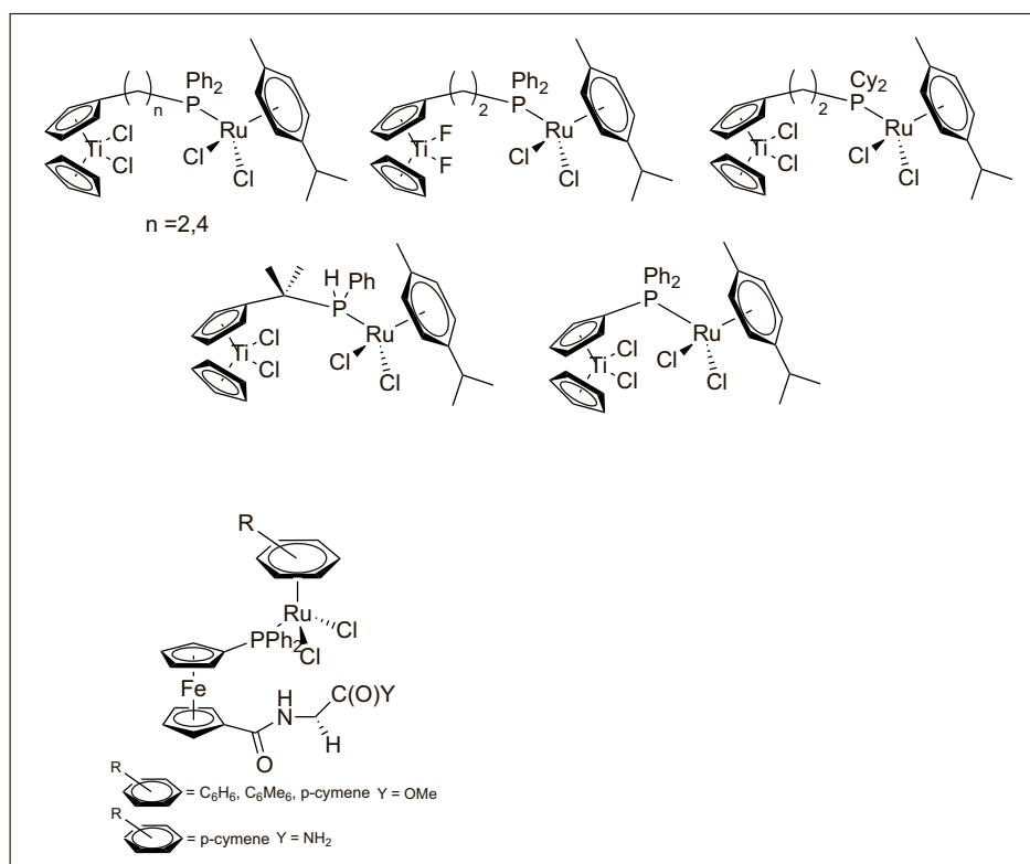
Fig. 10. Ferrocene and titanocene dichloride complexes conjugated to a [Ru(η 6 -arene)Cl 2 ] frame via a phosphine ligand.
