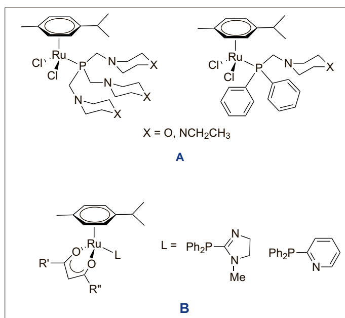
Fig. 4. Ru(II) p -cymene compounds with: a) aminomethylphosphines; b) aminophosphines.
