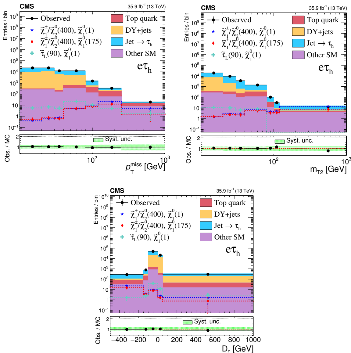
Figure 5. Distributions of the search variables p_T^{\text{miss}} (top left), m_{T2} (top right), and D_\chi (bottom) for the e\tau_h final state for events after the baseline selection. The black points show the data. The background estimates are represented with stacked histograms. Distributions for two benchmark models of chargino-neutralino production, and one of direct left-handed \tilde{\tau} pair production, are overlaid. The numbers within parentheses in the legend correspond to the masses of the parent SUSY particle and the \tilde{\chi}_1^0 in GeV for these benchmark models. In all cases, the last bin includes overflows.
