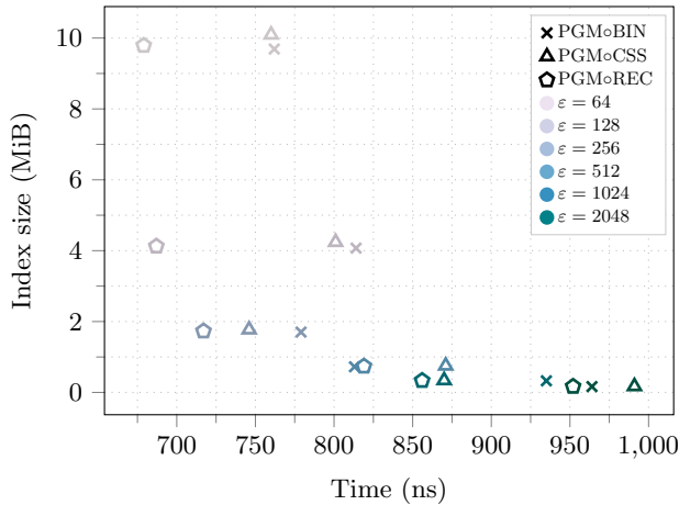
Figure 4: The (recursive) PGM-index, depicted as a pentagon, had better space and time performance than all the other configurations. For \epsilon > 256 all the three configurations behaved similarly because the index was so small to fit into the L2 cache.
