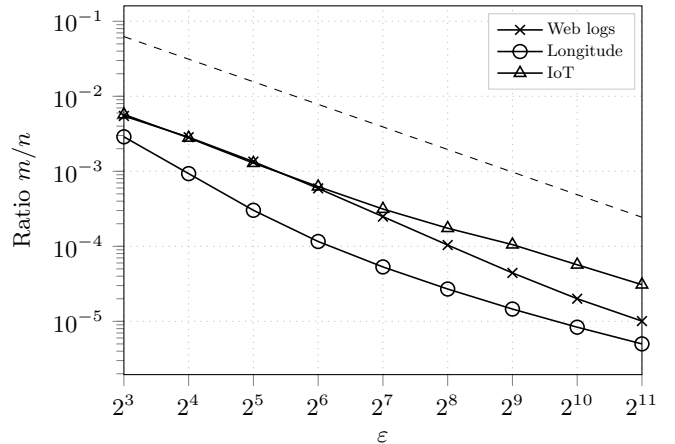
Figure 3: A log-log plot with the ratio between the number of segments m , stored in the last level of a PGM-index, and the size n of the real-world datasets as a function of \varepsilon . For comparison, the plot shows with a dashed line the function 1/(2\varepsilon) which is the fraction of the number of keys stored in the level above the input data of B^+ -tree with B = 2\varepsilon (see text). Note that m is 2–5 orders of magnitude less than n .
