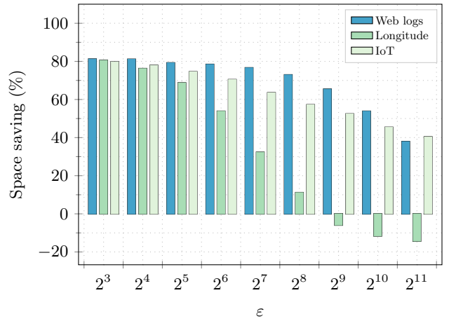
Figure 7: Slope compression reduces the space taken by the slopes up to 81.2%. Longitude is the only dataset on which compression does not help for \varepsilon \geq 2^9 because of its special features.
