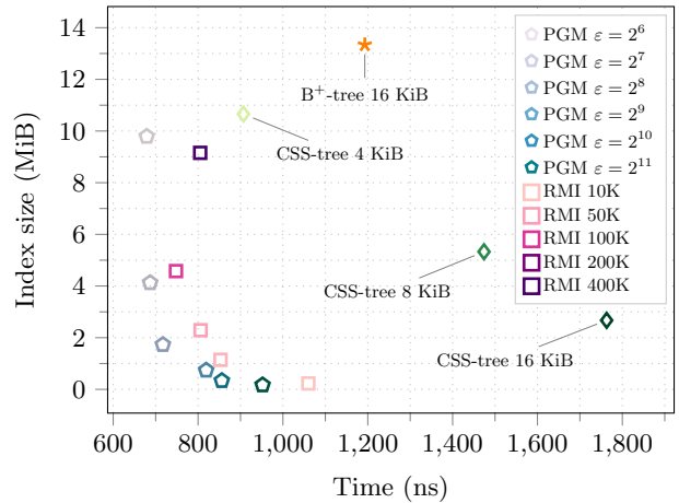
Figure 5: The PGM-index improved uniformly RMI with different second-stage sizes and traditional indexes with different page sizes over all possible space-time trade-offs. Results of traditional indexes for smaller page sizes are not shown because too far from the plot range. For example, the fastest CSS-tree occupied 341 MiB and was matched in performance by a PGM-index of only 4 MiB (82.7 \times less space); the fastest B^+ -tree occupied 874 MiB and was matched in performance by a PGM-index which occupied only 87 KiB (four orders of magnitude less space). The construction times of CSS-tree and PGM-index were similar (1.2 and 2.1 seconds, respectively), whereas RMI took 30.4 seconds (14.5 \times more than the PGM-index).
