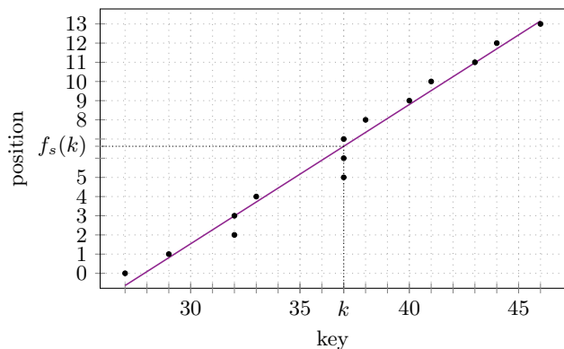
Figure 1: Linear approximation of a set of keys in the range [27, 46]. The function f_s is defined by two floats, and thus its storage is independent of the number of “covered” keys. The key k = 37 is repeated three times in the set, and f_s errs by \varepsilon = 2 in predicting the position of its first occurrence. Hence a search in a neighbourhood of size \varepsilon is enough to find the correct position of k .
