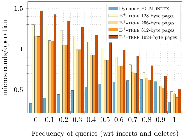
Figure 6: The Dynamic PGM-index was 13–71% faster than the B + -tree in the vast majority of workloads, with only a slight loss in the read-heavy case with 90% queries and 10% inserts/deletes. Overall, it improved the space of the four B + -tree configurations by 3891×, 2051×, 1140×, 611×, respectively.
