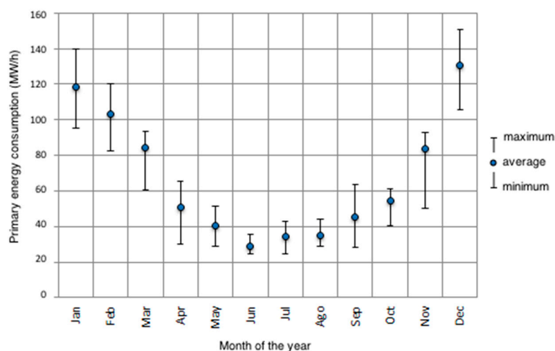
Figure 4. Trend of the average annual consumption of primary energy.
