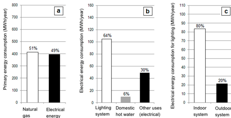
Figure 6. Distribution of the calculated consumptions: (a) Primary energy; (b) Electrical energy; and (c) Electrical energy used for lighting.
