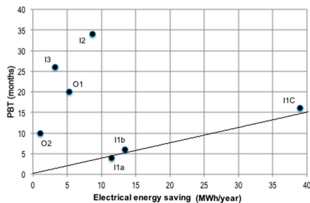
Figure 8. PBT values (months) vs. electrical energy saving (MWh/year) for the seven analysed interventions on the indoor and outdoor lighting systems.
