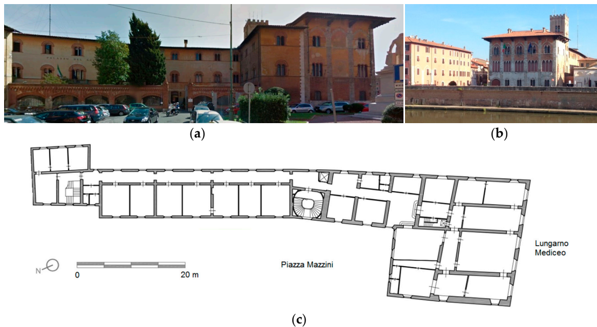
Figure 2. Palazzo Medici in Pisa: (a) Western front view; (b) Southern front view; and (c) A schematic plan of the second floor.
