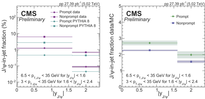
Fig. 2. Left: The fraction of prompt and nonprompt J/\psi in jets of 25 < p_T < 35 \text{ GeV} in pp data and in PYTHIA 8, compared to the total number of J/\psi in the relevant the p_T interval, as indicated on the Figure. Right: The ratio of these J/\psi -in-jet fractions in data compared to simulation for prompt and nonprompt J/\psi [5].
