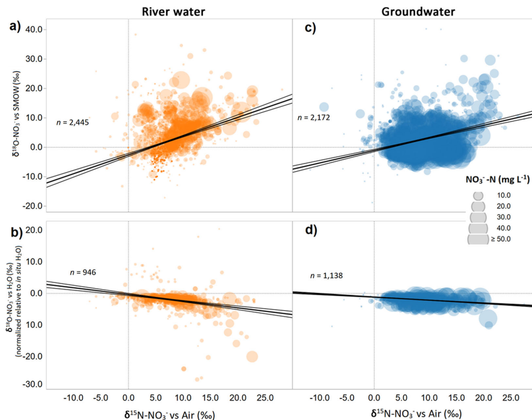
Fig. 2 \delta^{18}\text{O} vs \delta^{15}\text{N} of \text{NO}_3^- in rivers and groundwater. Symbol size denotes \text{NO}_3^- -N concentration in \text{mg L}^{-1} . The \delta^{18}\text{O} values are relative to SMOW and normalized to in situ \text{H}_2\text{O} , as described in Venkiteswaran et al. 31 . The results of the linear regression models of panels a–d are in Supplementary Table 4.
