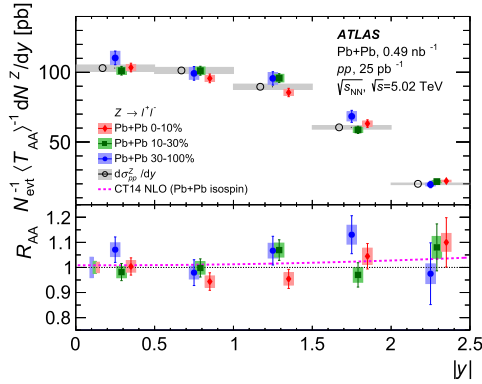
Fig. 4. Normalised Z boson yield versus rapidity measured in three centrality intervals: peripheral 30–100% (blue circles), mid-central 10–30% (green squares) and central 0–10% (red diamonds). The differential Z boson cross sections measured in pp collisions are shown by open circles [15]. The error bars on the data points indicate the statistical uncertainties and the shaded boxes show the total systematic uncertainties. The lower panel shows the R_{AA} and the contribution from the isospin effect calculated with CT14 NLO PDF (dashed line). The shaded boxes at unity indicate the combined uncertainty from the pp data added in quadrature to the T_{AA} uncertainty. The points in each centrality interval are shifted horizontally relative to the bin centre for clarity.
