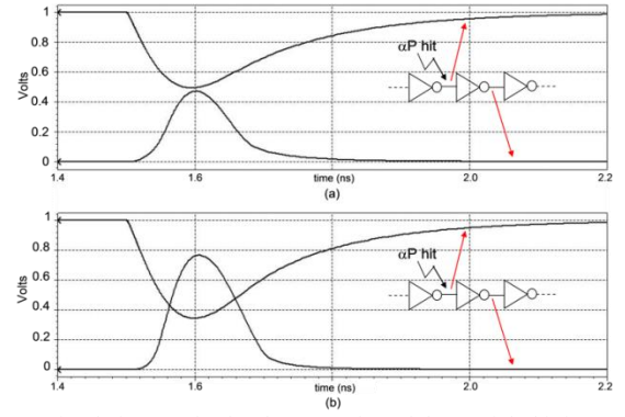
Fig. 1. Simulation results for the case of an alpha particle hitting a node of a NOT chain: (a) at the beginning of circuit operation; (b) after 10 years of circuit operation.
