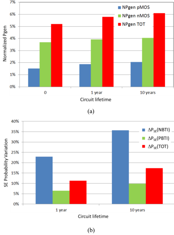
Fig. 5. (a) Alpha particle induced voltage glitch generation probability; (b) SE probability relative variation.
