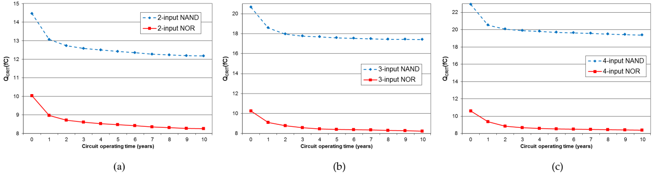
Fig. 3. Worst case Q_{crit} as a function of circuit lifetime, for NANDs (dashed lines) and NORs (solid lines) with 2 (a), 3 (b) and 4 (c) inputs.
