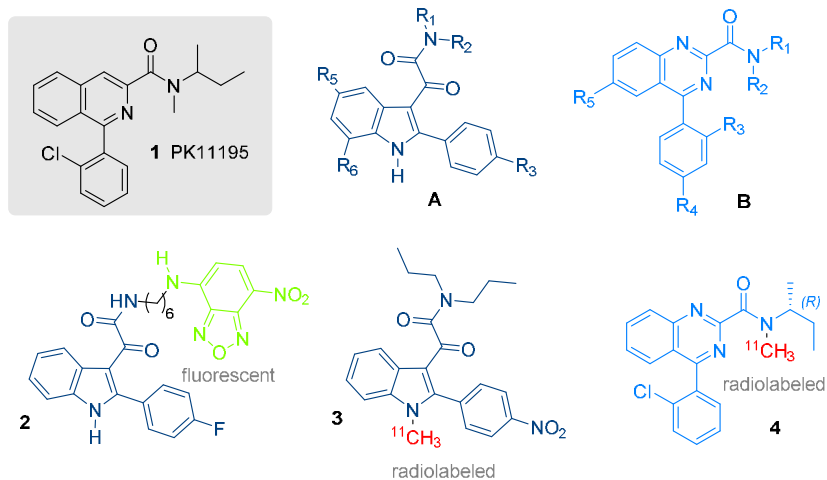
Chart 1. General structure of 2-arylindol-3-glyoxylamides ( A ) 19-21 and 4-phenylquinazoline-2-carboxamides ( B ), 23,24 together with 1 and fluorescent ( 2 ) 25,26 and radiolabeled ( 3 , 4 ) 27-29 probes belonging from classes A and B .
