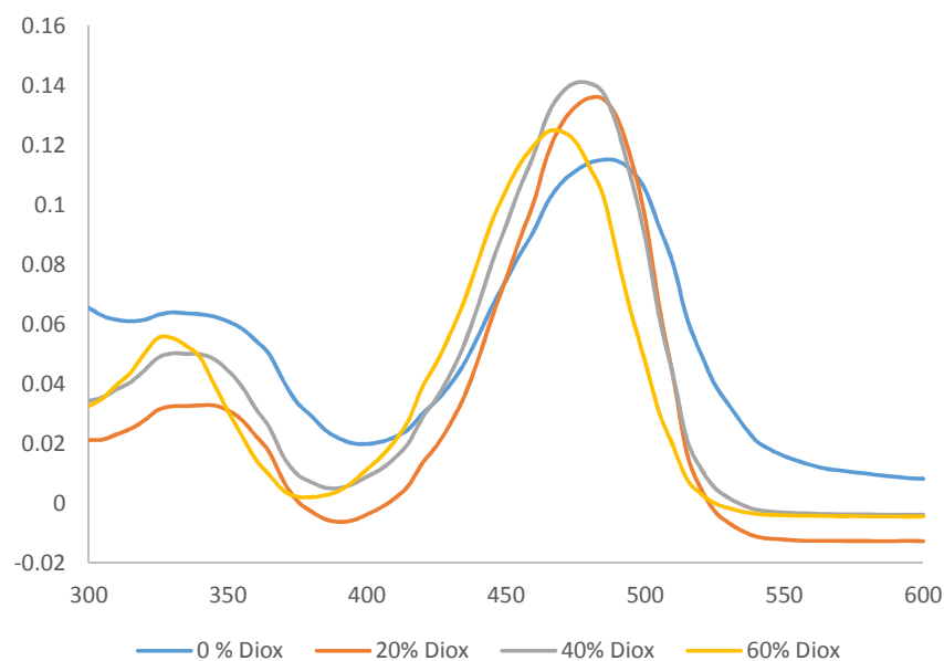
14 15 16 17 18 19 20 21 22 23 24 25 26 27 28 29 30 31 32 33 34 35 Figure 2. Absorption spectra of compound 15 at 10 \mu\text{M} in solutions varying from aqueous to 60% 36 dioxane-water (v/v) PBS. 37 38
