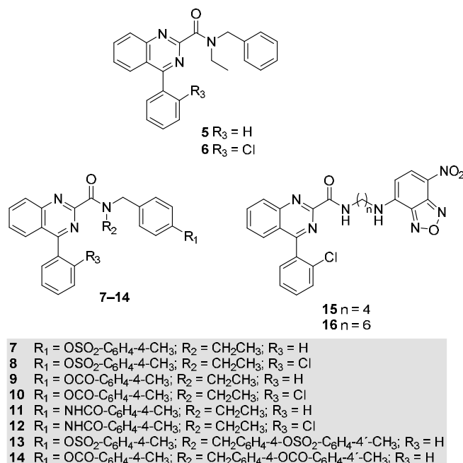
Chart 2. General structure of 4-phenylquinazoline TSPO ligands ( 5-14 ) and fluorescent probes ( 15, 16 ).
