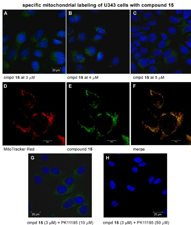
34 Figure 4. Compound 15 specifically labels mitochondria of human glioblastoma cell line U343. 35 Panels A–C: U343 cells stained with 15 (3, 4 and 5 \mu\text{M} ); panels D–F: comparison of U343 cells 36 stained with mitochondria specific dye MitoTracker Red (D) and with compound 15 (E) and 37 merged image (F); panels G, H: human glioblastoma cell line U343 stained with 15 (3 \mu\text{M} ) in the 38 presence of 1 (10 and 50 \mu\text{M} , respectively). 39 40 41 42
