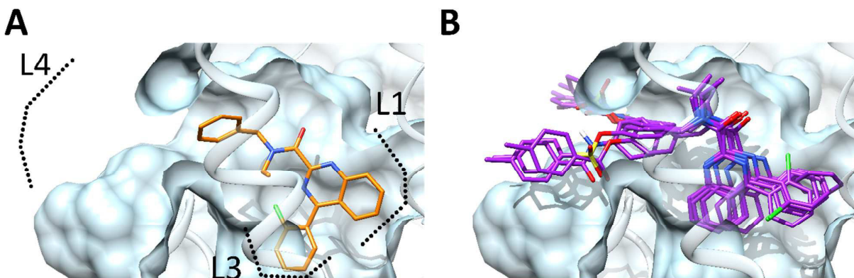
Figure 1. Binding mode of compound 6 (panel A, orange sticks) and 7-12 (panel B, purple sticks) into the rTSPO binding site (cyan ribbons and surface). In panel (A) the three receptor clefts identified from the topological model are also outlined.
