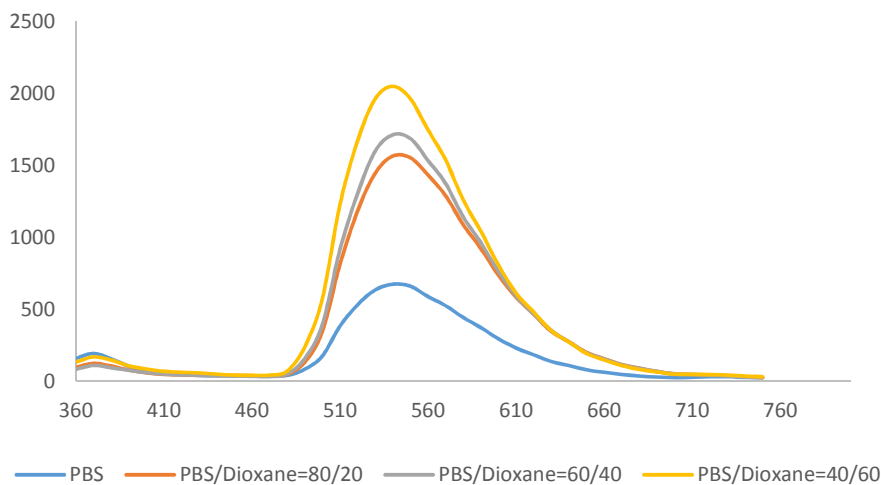
33 34 35 36 37 38 39 40 41 42 43 44 45 46 47 48 49 50 51 52 53 54 55 56 57 58 59 60 Figure 3. The influence of the polarity of the medium on the fluorescence of compound 15 was investigated by the addition of dioxane (indicated in % v/v) in PBS measured at a \lambda_{\text{max}} of 470 nm.
