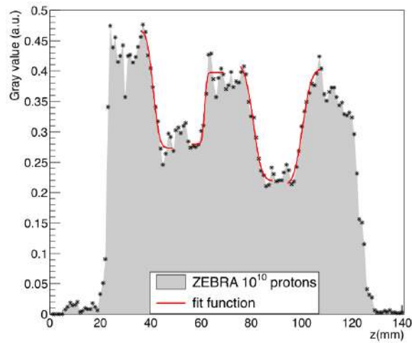
Figure 4: Activity profiles of ZEBRA phantom obtained with 10^{10} protons: the edges of the activity deficits corresponding to the presence of BRAIN slabs are fitted with error functions (red).
