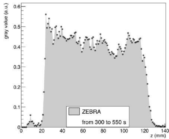
Figure 5: Activity profiles of ZEBRA phantoms obtained with 10^{10} protons: the edges of the activity deficits corresponding to the presence of BRAIN slabs are fitted with error functions. Profile is obtained integrating the signal in the [300, 550] s time window.
