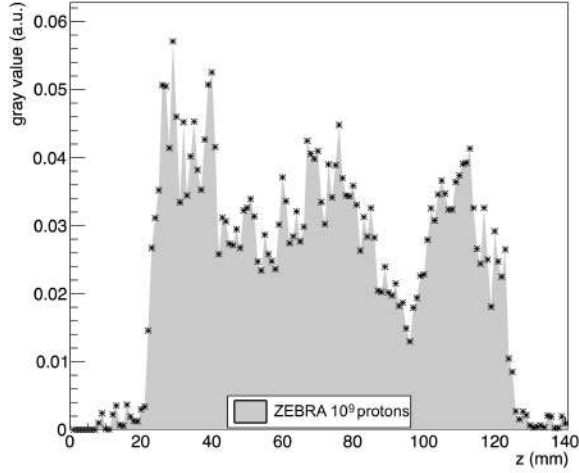
Figure 6: Activity profiles of ZEBRA phantom obtained with 10^9 protons in the [0, 120] s time window: it is not possible to clearly identify the presence of BRAIN slabs.
