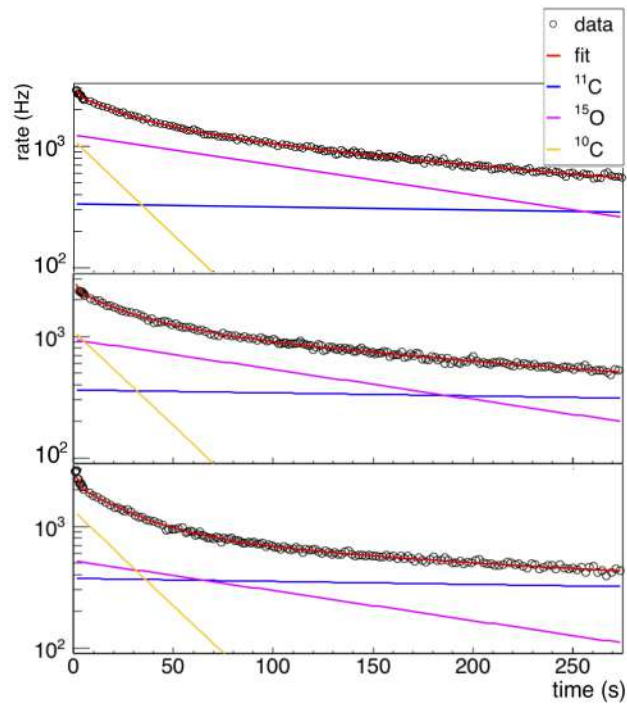
Figure 8: Zoom view for the coincidence rate in [0, 270] s time window. Top: PMMA homogeneous phantom. Central: ZEBRA phantom. Bottom: BRAIN homogeneous phantom.
