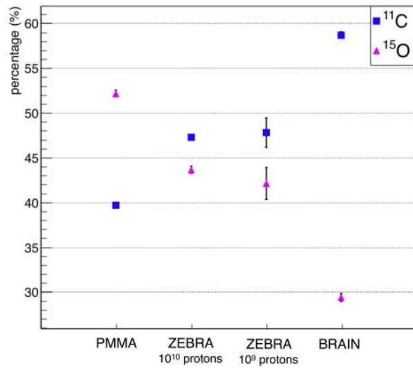
Figure 9: Percentages of ^{15}\text{O} and ^{11}\text{C} for all the studied irradiations.
