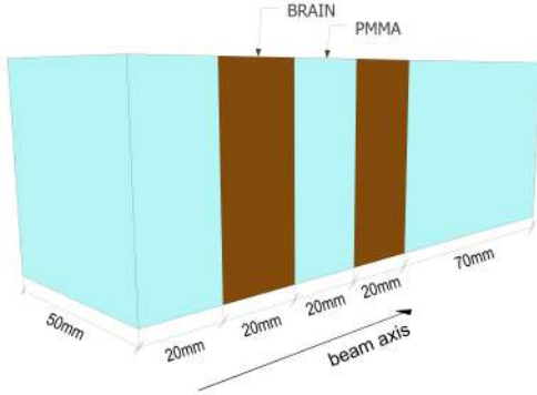
Figure 1: 3D view of ZEBRA phantom: light blue slabs are PMMA, brown slabs are BRAIN.
