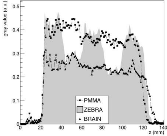
Figure 3: Activity profiles of PMMA, ZEBRA and BRAIN phantoms irradiated with 10^{10} protons: the z coordinate corresponds to the beam axis. Square points refers to PMMA, triangles to BRAIN and grey area to ZEBRA phantom. Profiles are obtained integrating the signal in the (0, 120 s) time window.
