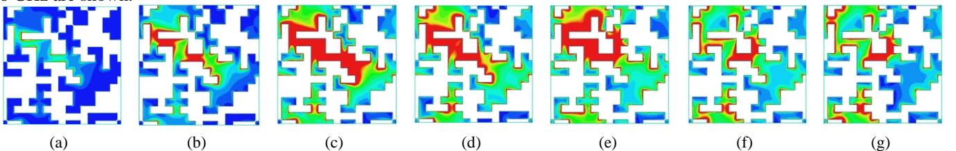
Fig. 5 – Surface current distribution of the unit cell obtained at the end of the optimization process calculated at 4\text{ GHz} (a), 6\text{ GHz} (b), 8\text{ GHz} (c), 16\text{ GHz} (d), 26\text{ GHz} (e), 34\text{ GHz} (f) and 36\text{ GHz} (g).
