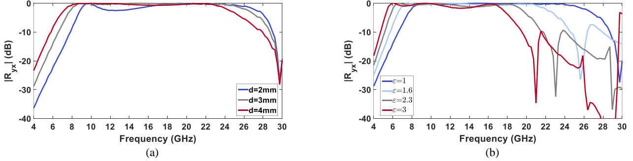
Fig. 3 – |R_{yx}| as a function of the frequency for an air substrate of thickness d = 2\text{ mm}, 3\text{ mm}, 4\text{ mm} (a); |R_{yx}| as a function of the frequency for a loss less substrate with a thickness of 3\text{ mm} for \epsilon = 1, 1.6, 2.3, 3 (b).
