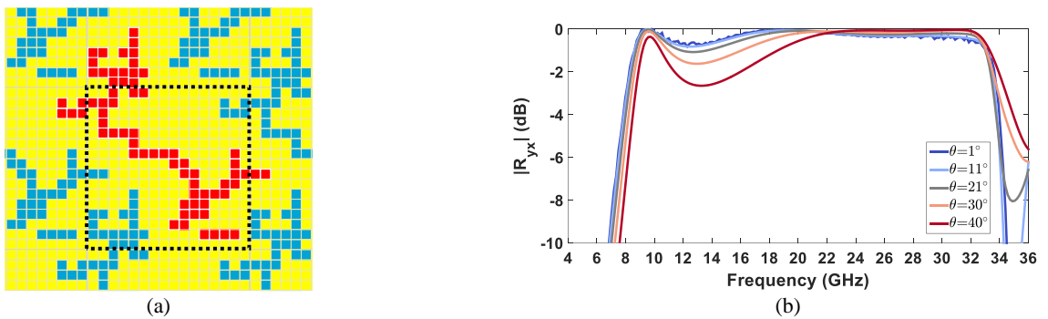
Fig. 9 – Metasurface's topology: the resonant element (highlighted in red) extends beyond the minimum period of the metasurface (black dotted line) (a); Simulated |R_{yx}| of the refined metasurface as a function of the frequency for different elevation angles ( \theta = 1^\circ, 11^\circ, 21^\circ, 30^\circ, 40^\circ ) of the incident wave (b).
