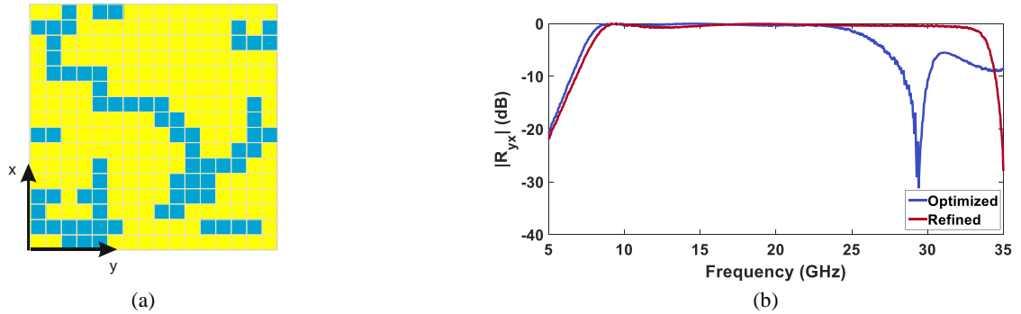
Fig. 7 – (a) Refined unit cell; (b) |R_{yx}| as a function of the frequency for the original and refined unit cell.
