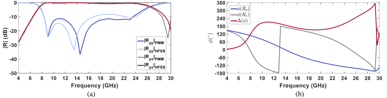
Fig. 4 – |R_{yy}| and |R_{yx}| as a function of the frequency calculated by the PMM and by HFSS (a); (b) Phase of the reflection coefficient \phi(R_u) and \phi(R_v) and phase difference \Delta(\phi) = \phi(R_u) - \phi(R_v) as a function of the frequency calculated by the PMM.
