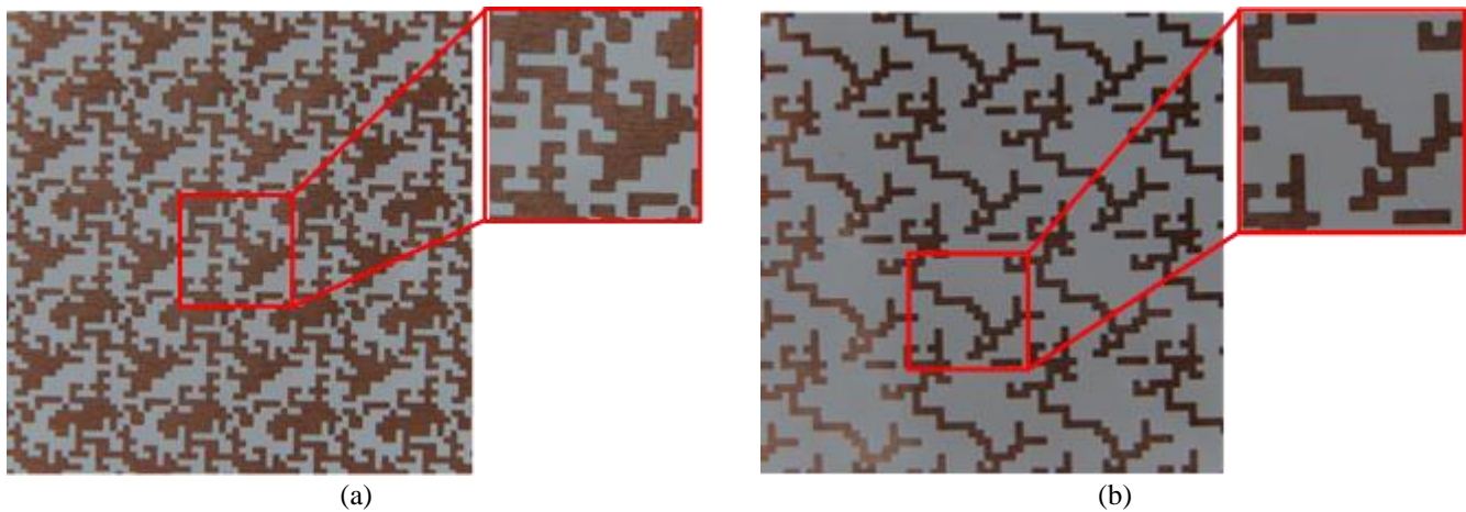
Fig. 11 – GA-optimized (a) and refined (b) prototype fabricated with the photolithographic process. The zoom view of the unit cell is shown in the inset.
