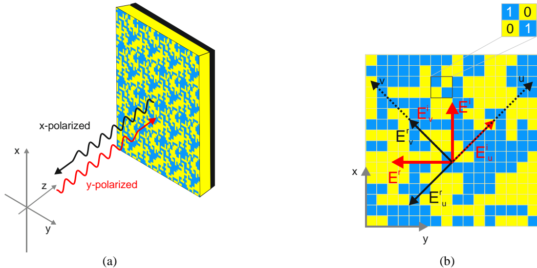
Fig. 1 – (a) Reflective linear polarization converter geometry; (b) Representation of the incident electric field decomposition in the uv -coordinate system.
