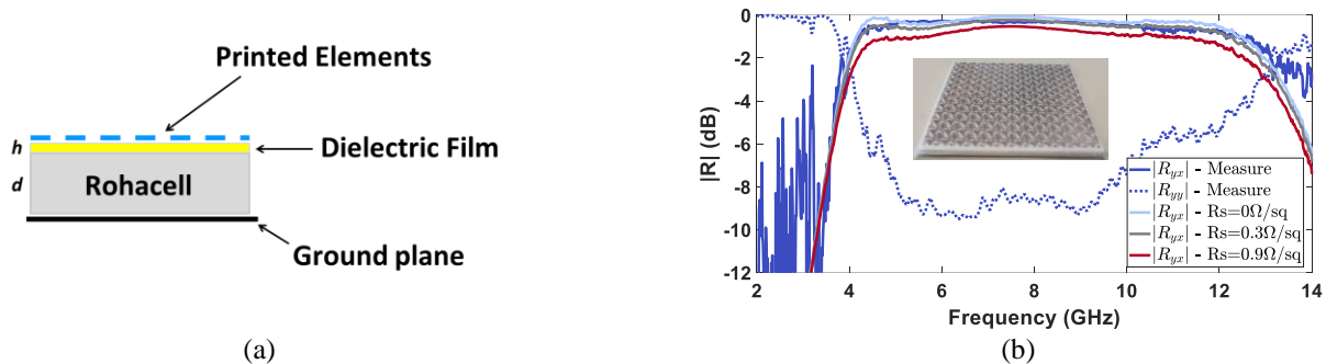
Fig. 10 – (a) Stack-up of the polarization converter; (b) Preliminary prototype: comparison between the measured |R_{yy}| and |R_{yx}| and the simulated |R_{yx}| as a function of the frequency for the for different values of the surface resistance R_s = 0, 0.3, 0.9 \Omega/\text{sq} .
