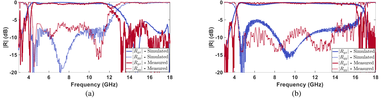
Fig. 12 – Comparison between the simulated and measured |R_{yx}| and |R_{yy}| as a function of the frequency for the GA-optimized (a) and refined (b) polarization converter.
