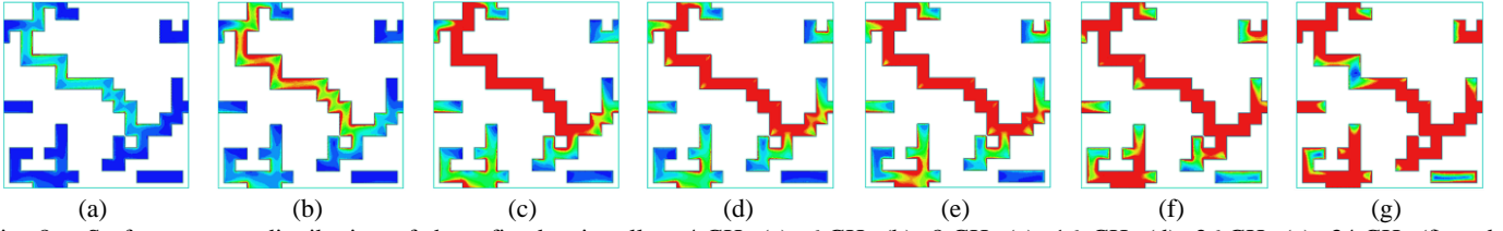
Fig. 8 – Surface current distribution of the refined unit cell at 4 GHz (a), 6 GHz (b), 8 GHz (c), 16 GHz (d), 26 GHz (e), 34 GHz (f) and 36 GHz (g)
