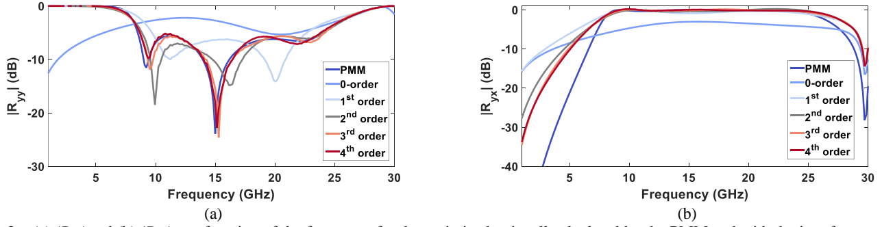
Fig. 2 – (a) |R_{yy}| and (b) |R_{yx}| as a function of the frequency for the optimized unit cell calculated by the PMM and with the interference theory approach extended up to the fourth order.
