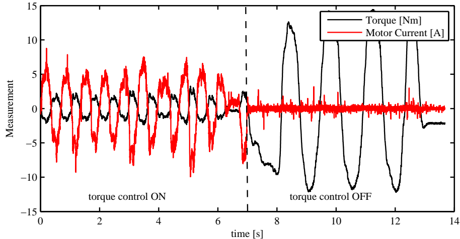
Figure 9: Initial zero torque control results.
