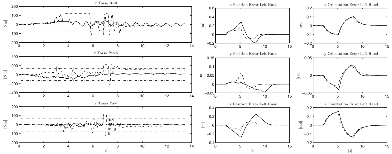
Figure 27: On the left, measured torques on the joints of the torso while performing the task without (dashed lines) and with (continuous lines) the robot dynamics constraint. The constant lines shows the limits on the torques. On the right, Cartesian error on the left hand while performing the task without (dashed lines) and with (continuous lines) the robot dynamics constraint
