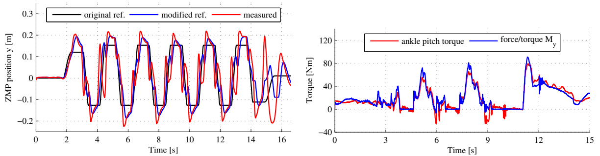
Figure 34: On the left lateral ZMP data from forward walking experiments. The black, blue and red lines represent the original ZMP reference of the planned motion, reference modified by the ZMP feedback controller and measured ZMP position, respectively. On the right comparison of torque measured by ankle pitch torque sensor and foot force/torque sensor.
