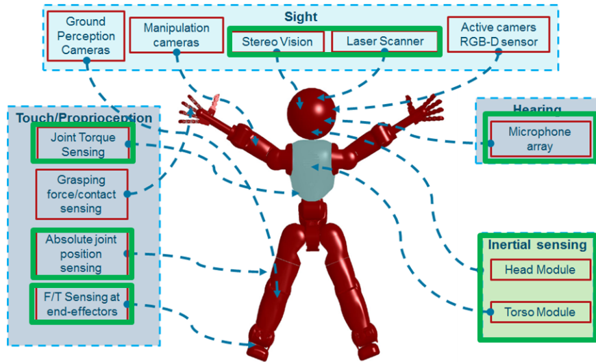
Figure 13: WALK-MAN perception system components.
