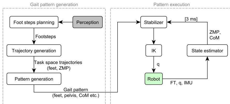
Figure 28: Locomotion control diagram.
