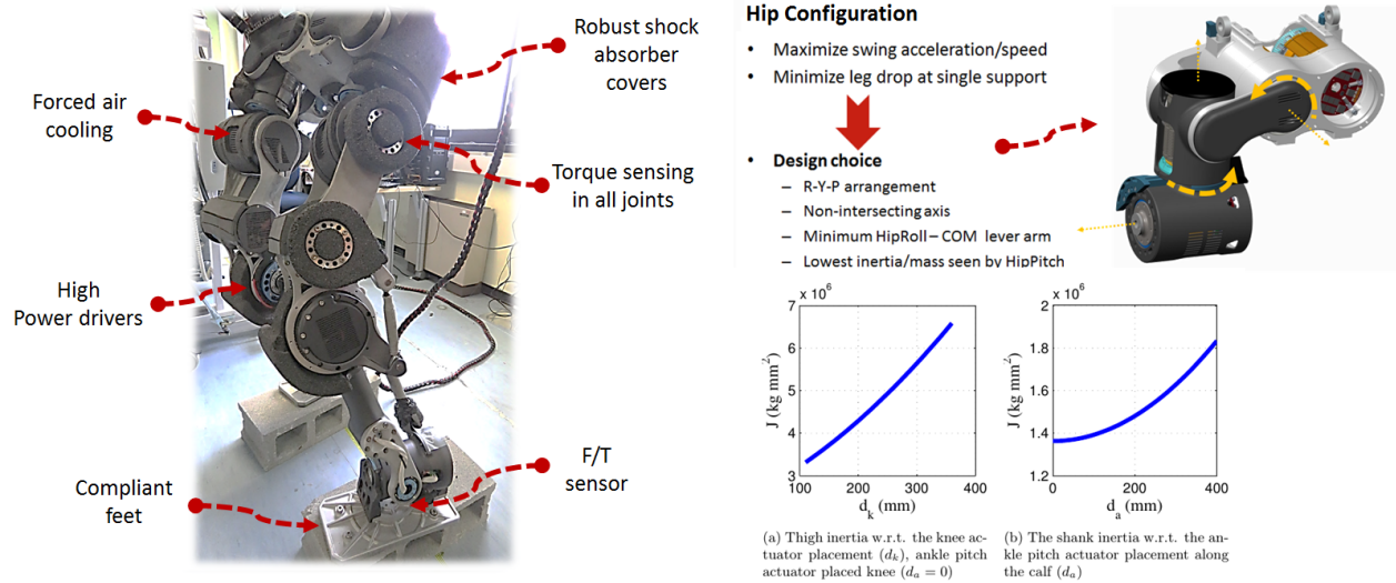
Figure 6: WALK-MAN leg features, Hip Configuration and effect of knee and ankle pitch actuators location on the leg inertia.
