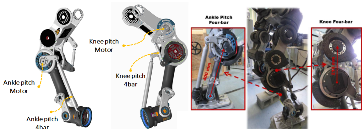
Figure 7: The relocation of knee and ankle pitch actuators and the 4-bar transmissions.
