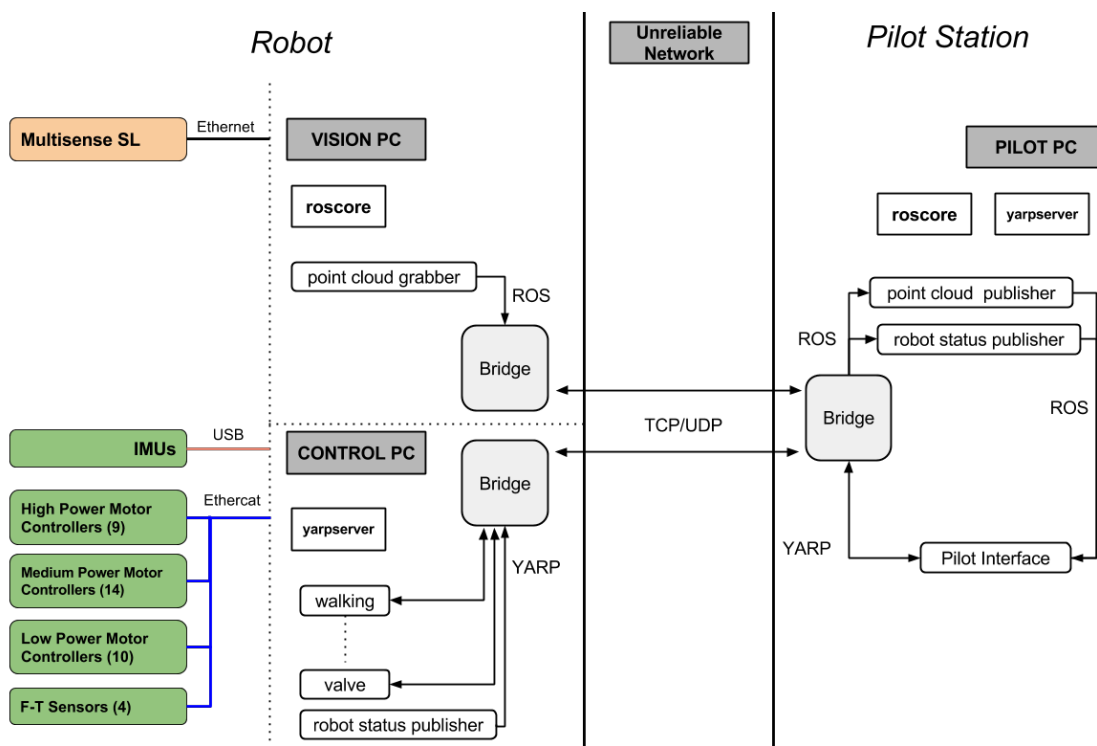
Figure 17: System PCs connections and interactions.
