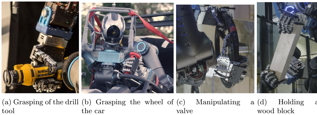
Figure 5: The adaptiveness, versatility and robustness of the hand employed in the execution of grasping and manipulation tasks.
