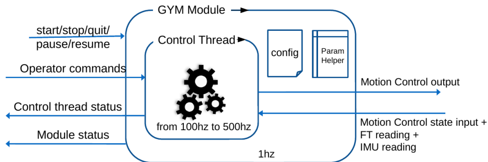
Figure 16: GYM (Generic Yarp Module) control thread and communication interfaces.
