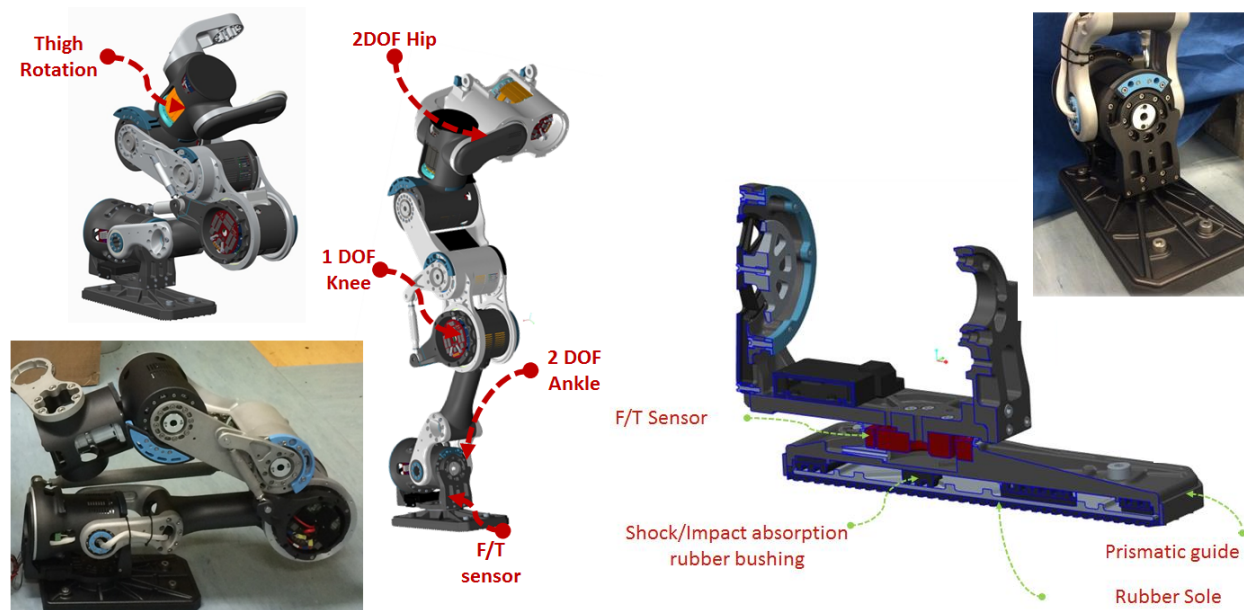
Figure 8: WALK-MAN Leg Kinematics and foot design.
