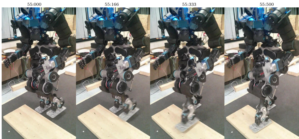
Figure 35: Snapshots from dynamic stepping on the obstacle. The obstacle is 5 cm high and the step time is 0.7 s. The digits above pictures represent time of the experiment in ss:mmm format.
