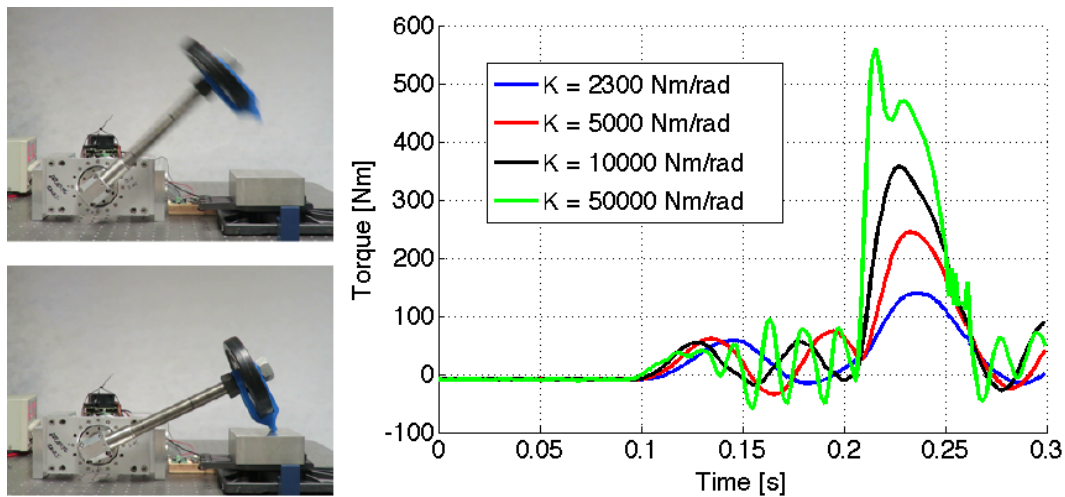
Figure 11: On the left the experimental setup used for the impact tests to demonstrate the effect of intrinsic compliance on the reduction of impact torques reaching the reduction drive. The test bed is composed by an actuation unit, a hammer system, a F/T sensor and rigid and soft covers with different stiffness. On the right impact torque profiles as a function of the compliance of the torsion bar.
