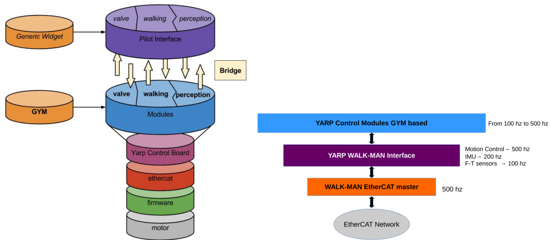
(a) Complete view of the software architecture. (b) Loop frequency of the different software layers.
