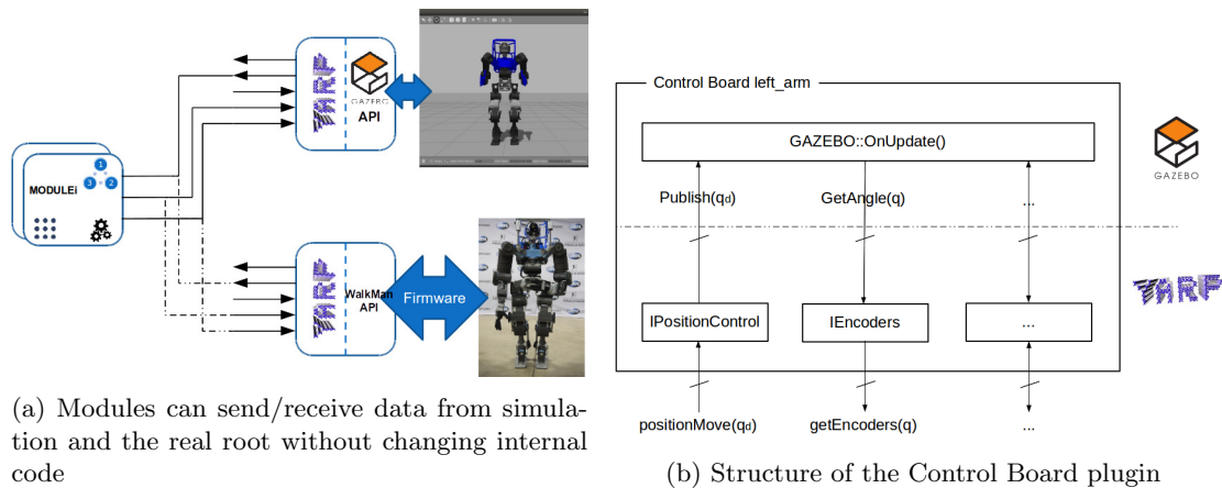
Figure 18: Simulator infrastructure
