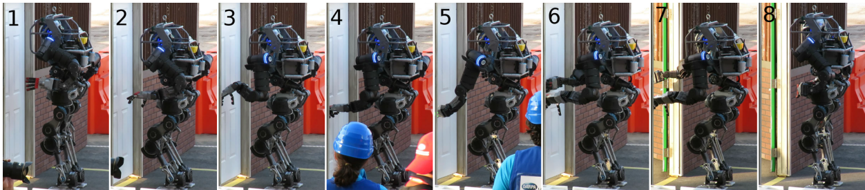
Figure 32: Door opening task execution in the DRC.
