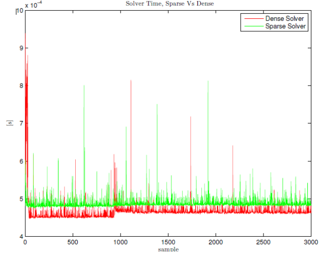
Figure 25: An example of stack description and the time needed to solve a stack of tasks, Sparse vs. Dense implementation, on an Intel Core i7. The problem has also two global constraints: keeping the Center of Mass inside the support polygon and keeping the velocity of the Center of Mass bounded) and two bounds (joint position and velocity limits)
