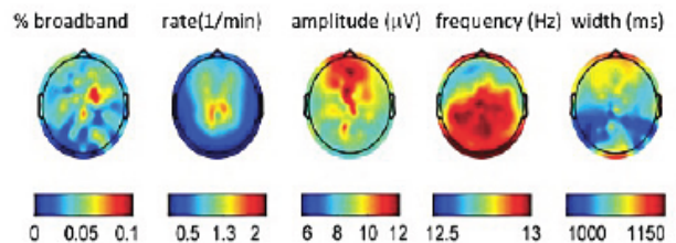
Fig. 3. Results - Group-averaged topological maps of spindle features.
