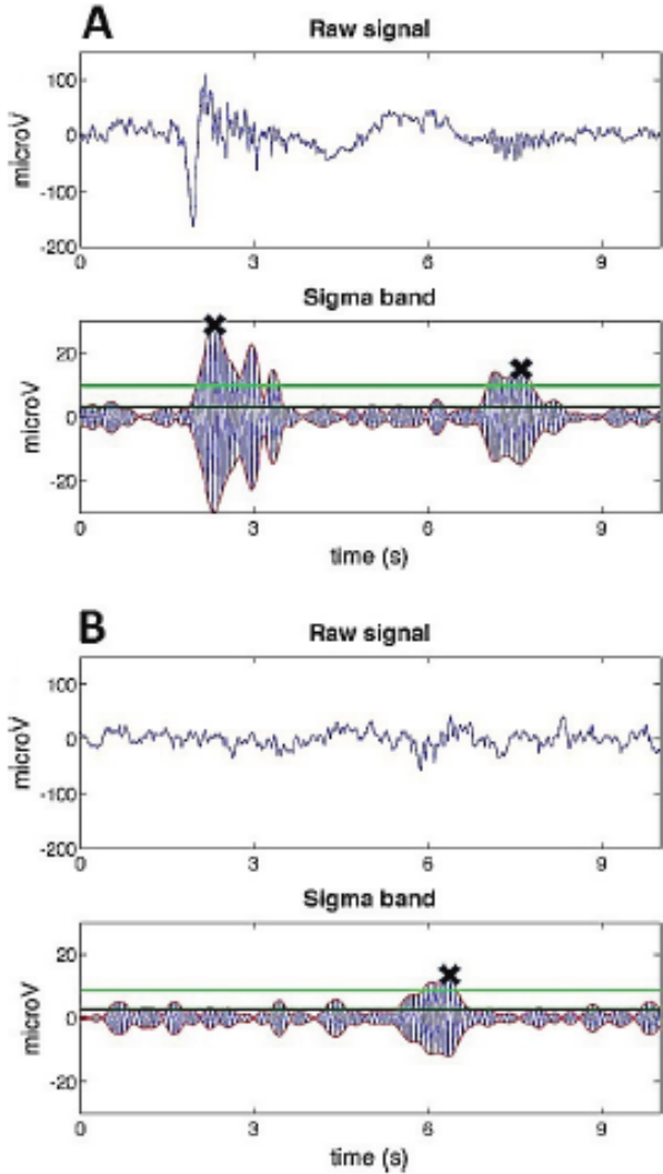
Fig. 2. Examples of spindle detection based on dynamic thresholds. Each panel has two traces: (top) The EEG signal, filtered in [0.5 - 40Hz] as usually seen during visual scoring - (bottom) EEG signal, filtered in [12 - 15Hz] . In red, the rectified signal, calculated via Hilbert Transform. In green, lower and upper thresholds. Panel A shows two full-fledged spindles. The first one is following a K-complex, the second one is an temporally isolated one. Both spindles would be recognized by visual scoring of any sleep expert. Panel B show a spindle warped by a slower oscillation and difficult to be identified during visual scoring.
