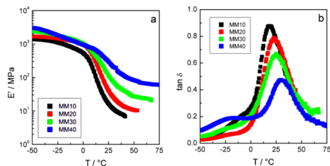
Figure 2. Trends of E' (a) and \tan \delta (b) for the films prepared by mixtures MM10-MM40 analyzed along the direction parallel to the liquid crystalline alignment.
