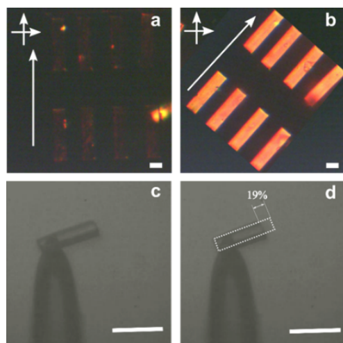
Figure 6. DLW blocks fabricated with MM10 mixture and their contraction under irradiation. a) and b) POM images of different blocks, respectively, parallel and at 45° in respect to the polarizer direction. The scale bar is 20 \mu\text{m} . c) and d) Optical image of a block suspended on a fiber, respectively, in the equilibrium position (no green laser excitation) and under a green laser light exposition. The scale bar is 80 \mu\text{m} .
