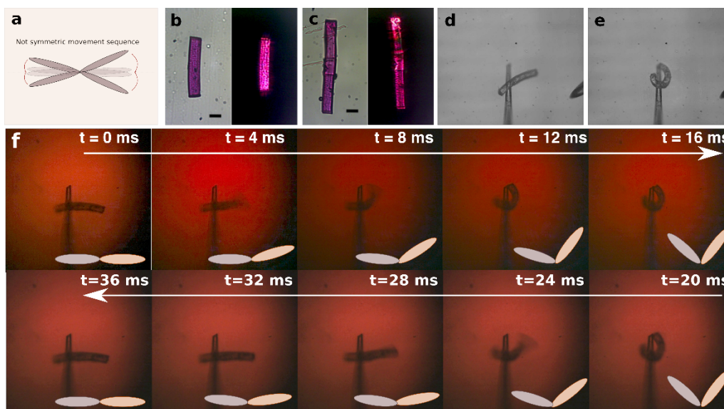
Figure 7. Fabrication and activation of a stripe with arms prepared by two different LCN mixtures ( MM10 and MM40 ). a) Scheme of a non-symmetric movement sequence (Ref. 17); b) A cantilever prepared by mixture MM40 in a splayed cell after development and its POM image demonstrating the LC alignment; c) A double materials stripe obtained after a second DLW process and development retaining the desired LC alignment as shown in POM images. The scale bar is 20 \mu\text{m} ; d) Optical image of a stripe suspended on a fibre, in the equilibrium position (no green laser light excitation) and e) under a green laser light irradiation; f) Sequence of fast camera video frames for the stripe bending and relaxation.
