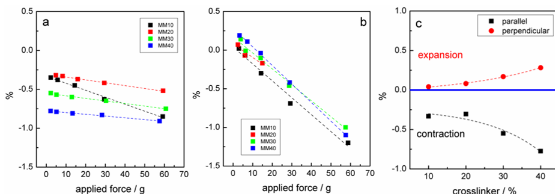
Figure 4. Effect of light irradiation on the deformation once the film were subjected to different total (static + dynamic) loads. Deformation as a function of the cross-linking degree in uniaxial planar films measured parallel (a) and perpendicular (b) to the director. Deformations % in length extrapolated at zero stress (c).
