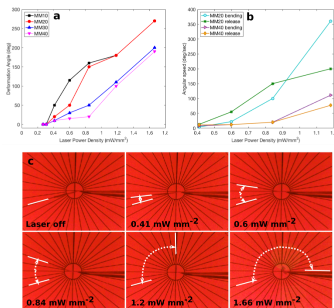
Figure 5. Response of splayed films to laser irradiation. a) Bending angle as a function of laser power for all mixtures; b) Angular speeds for MM20 and MM40 ; c) Photos showing splayed MM30 film response during irradiation at increasing laser power density.
