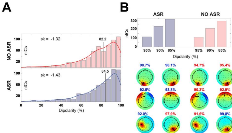
Fig. 3. ASR effect on ICA
