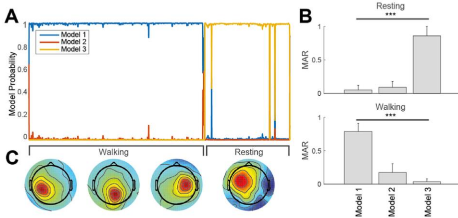
Fig. 9. Adaptive mixtures modeling
