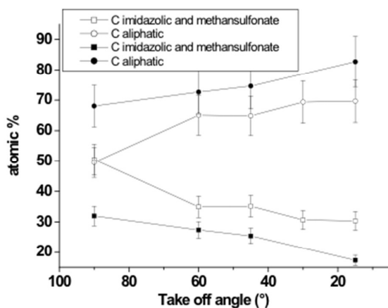
Fig 4. Contributes to the C 1s peak by aliphatic and imidazolium carbons as function of take-off angle for 5b (full symbols) and 5a (empty symbols) sample.
