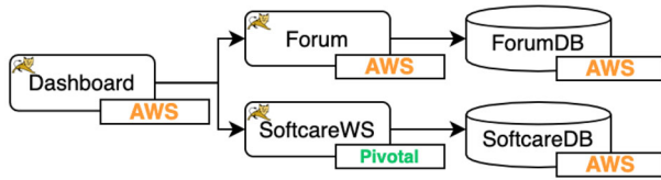
Fig. 1 Topology of the Softcare application
