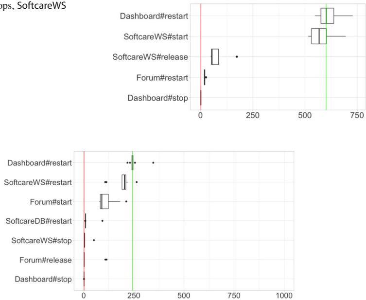
Fig. 10 Forum crashes and SoftwareDB stops
