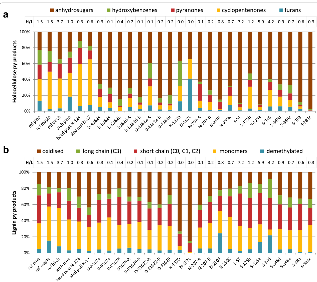
Fig. 5 Percentage distribution of a holocellulose and b lignin pyrolysis product categories in each sample; where the prefix D—Danish Dejbjerg, N—Norwegian Oseberg and S—Swedish Glimmingehus collection
