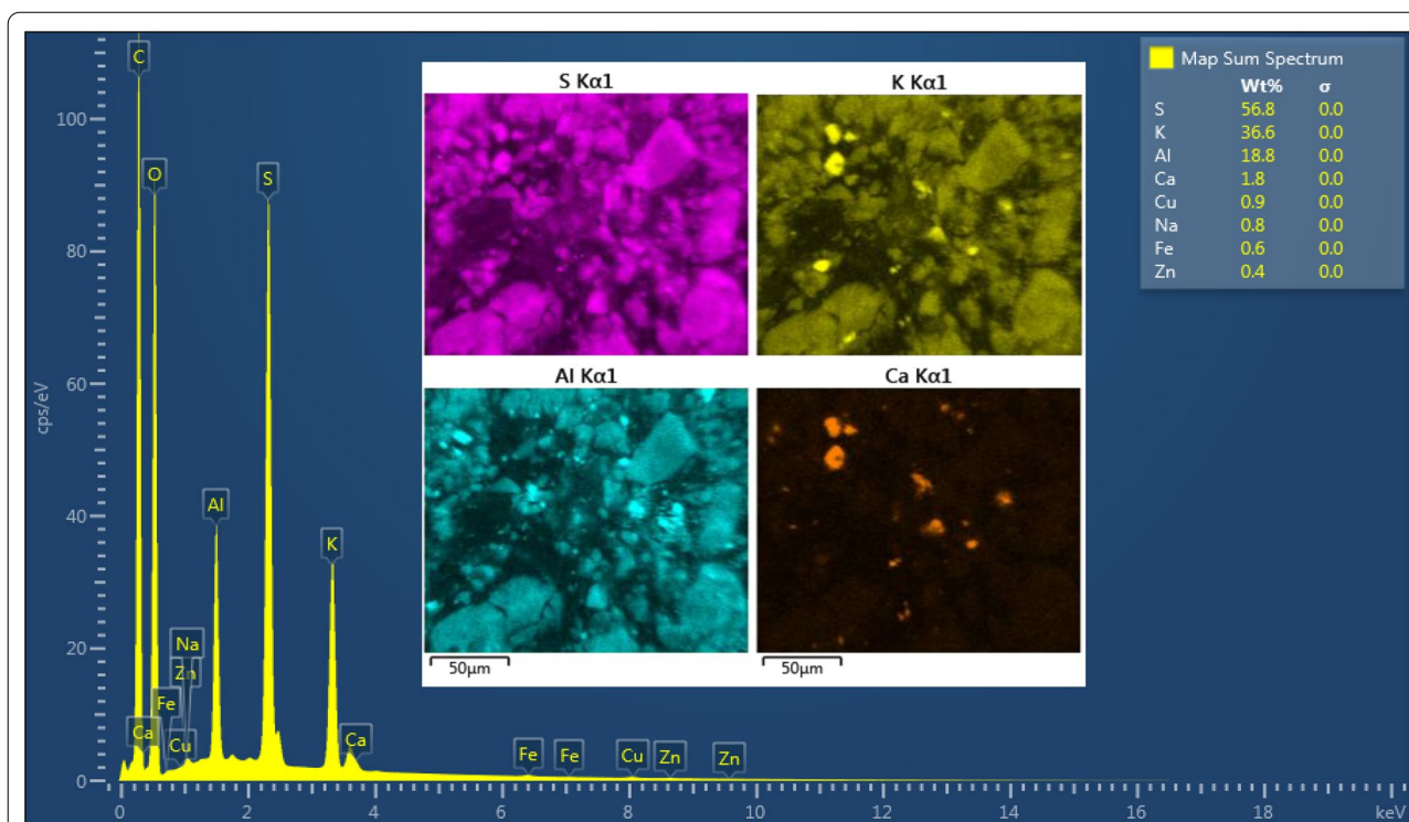
Fig. 3 SEM–EDS elemental maps of S, K, Al and Ca from sample D-C1628 showing the presence of K-alum as a major inorganic component and supporting the presence of the minor potassium calcium sulphate mineral syngenite
