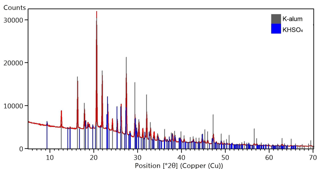
Fig. 1 X-ray diffraction pattern from sample N-187D (red), compared with \text{KHSO}_4 (blue) and potassium alum (grey) references
