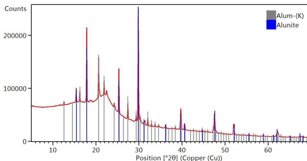
Fig. 2 X-ray diffraction pattern from sample N-250K (red) compared with alunite (KAl 3 (SO 4 ) 2 (OH) 6 , blue) and K-alum (grey) references
