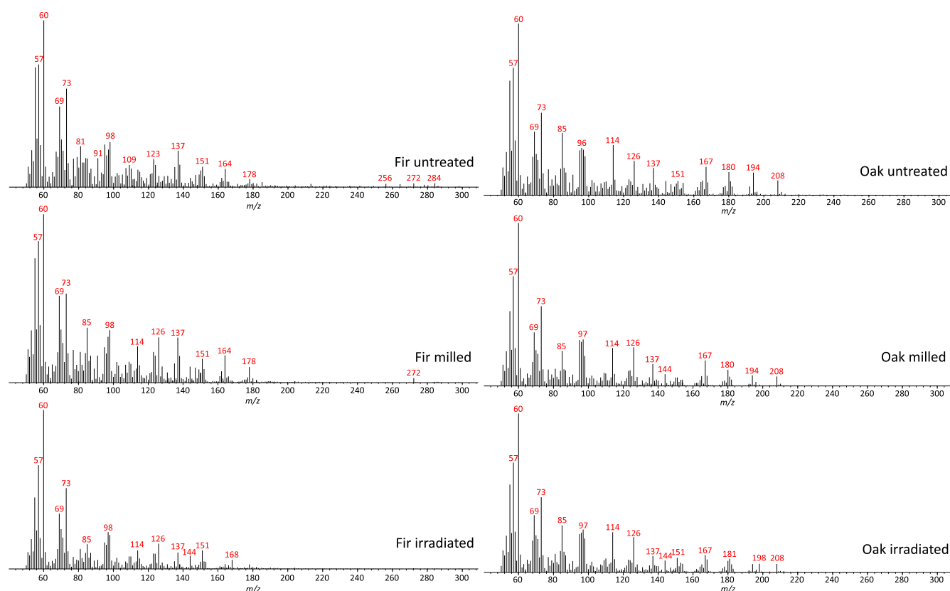
Figure 2. Average mass spectra from the EGA-MS profiles of fresh, milled, and irradiated fir and oak ( \beta = 20\text{ }^{\circ}\text{C/min} ).
