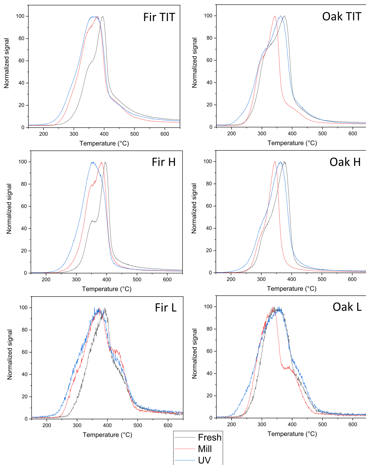
Figure 1. TIT and holocellulose (H) and lignin-specific (L) thermograms for fresh, milled, and irradiated fir and oak ( \beta = 20\text{ }^{\circ}\text{C}/\text{min} ).
