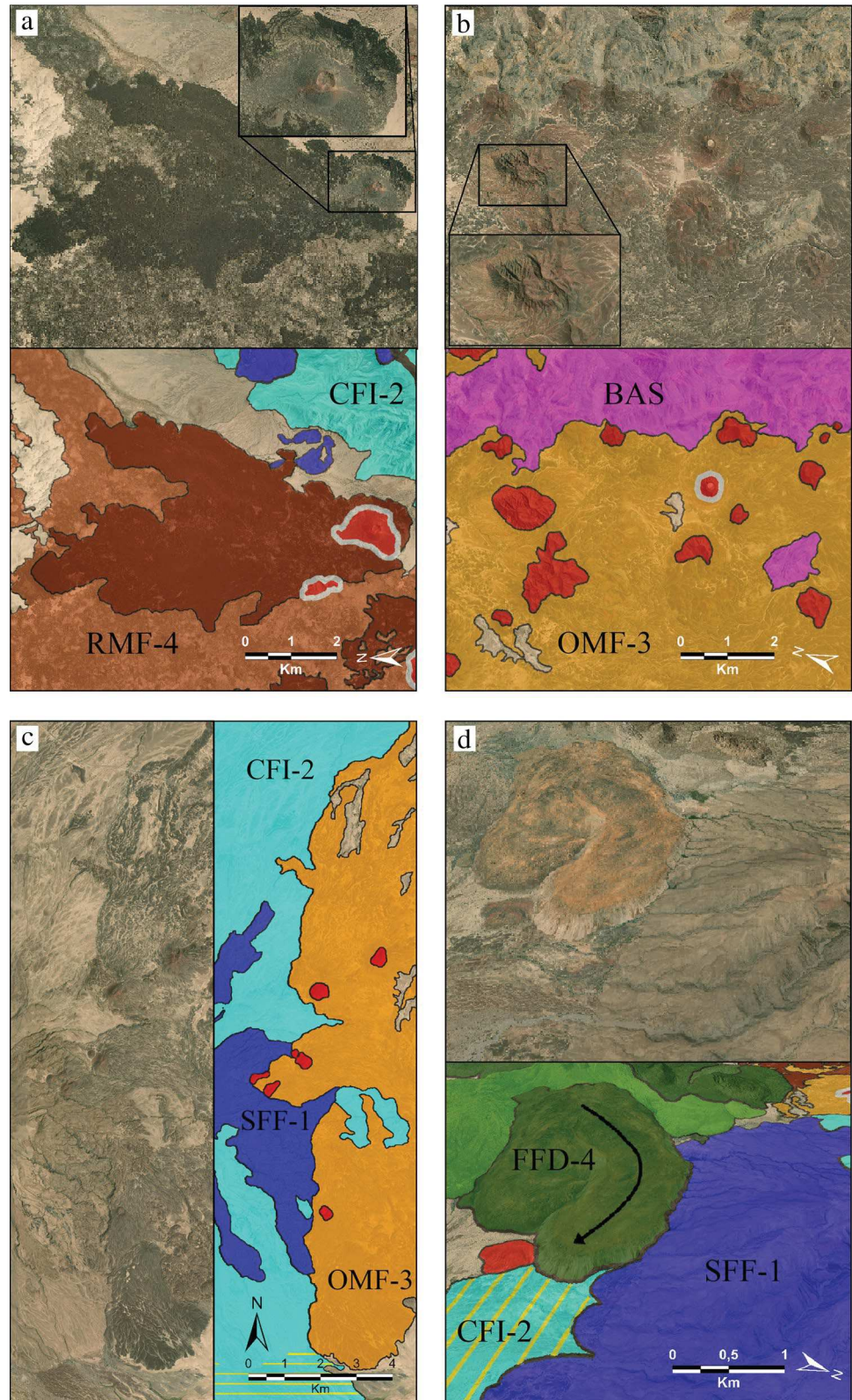
Fig. 5 Pairs of Landsat 5 satellite images and the relative geological map. SFF-1, stratovolcano felsic flows; CFI-2, calderas felsic ignimbrites; OMF-3, old mafic flows; RFM-4, recent mafic flows; FFD-4, felsic flows and domes; BAS basement. Locations are shown in online resource Fig. 6. World Imagery Source as in Fig. 2
