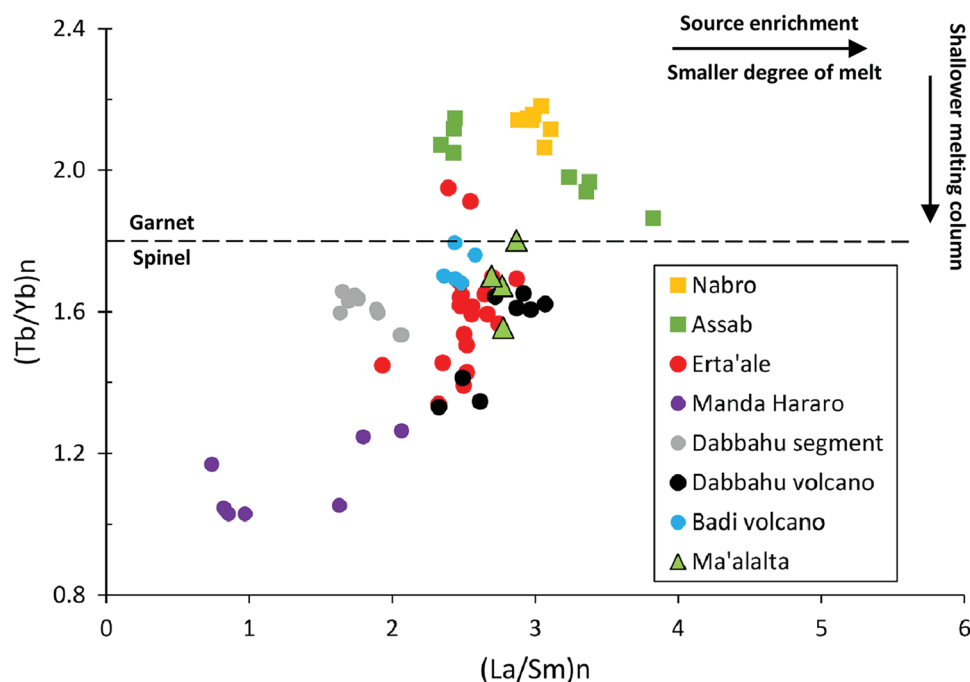
Fig. 9 Plot of \text{Tb}/\text{Yb} and \text{La}/\text{Sm} normalized to chondritic values (McDonough and Sun 1995). Only samples with \text{MgO} greater than 4 wt% are plotted. The division between spinel and garnet-dominated melting is derived from magma modelling in the Basin and Range province (Wang et al. 2002). As a comparison with the MVF, volcanism of different locations of the Afar region is shown: the marginal Nabro volcano (Donovan et al. 2018) and the transverse Assab range
