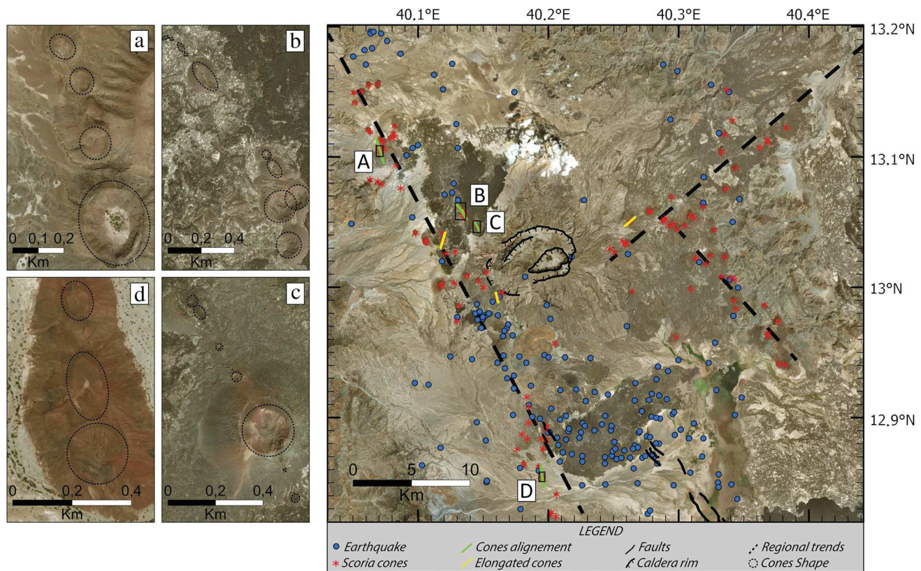
Fig. 8 Distribution of earthquakes (blue dots), cinder cones (red asterisks) and faults (solid black lines) of the MVF. a-d Elongated (351° E, 347° E, 17° E, 336° E and 321° E) and aligned (343° E, 327° E, 331° E and 351° E) cones (black dotted line). World Imagery Source as in Fig. 2
