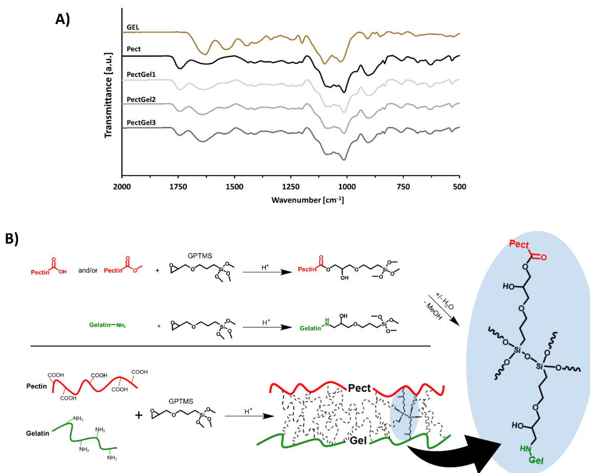
Figure 1 (A) ATR-IR spectra of PectGel1, PectGel2 and PectGel3, Pect and GEL, (B) Hypothetical crosslinking reaction mechanism in an aqueous environment; in an acidic environment, as generated by pectin, the GPTMS epoxide ring is opened and the resulting hydroxyl groups react with the carbonyl groups of pectin. [3] Concomitantly, an acid-catalyzed epoxide ring-opening occurs by primary amines on gelatin [28,29] . The two reactions lead to GPTMS residues linked by esters to pectin and linked by secondary amines to gelatin. Subsequently, in an aqueous environment, hydrolysis of the trimethoxysilane groups occurs (expulsion of methanol) followed by a condensation reaction forming Si-O-Si-linkages between polymer chains [30] . It must be noted that the reactions linking GPTMS to both polymers occur simultaneously in our system and are likely to compete. Which reaction is dominant and whether one of the reaction products is formed in majority, is still under investigation.
