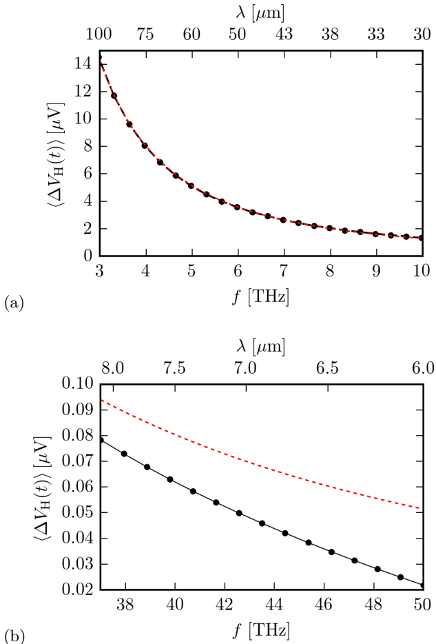
FIG. 4. (Color online) Hall voltage at large drive frequencies. In both panels (a) and (b), the red dashed line corresponds to the analytical estimate in Eq. (1) while the black circles correspond to the numerical solution of Eqs. (13) for vanishing viscosity \nu = 0 . The bottom axis shows the value of the drive frequency f and the top axis the corresponding value of the wavelength \lambda . (a) Frequencies in the far-infrared range. (b) Frequencies in the MIR range. Despite its drop in magnitude at large frequencies, the Hall voltage is measurable even in the MIR frequency range. The relative deviation between the analytical estimate and the numerical solution is \simeq 0.0016 at f = 3 THz and \simeq 1.3 at f = 50 THz.
