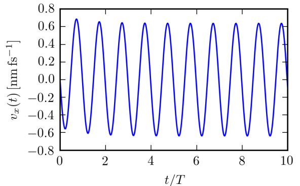
FIG. 3. (Color online) Time-evolution of the components of the velocity \mathbf{v}(y, t) , obtained from the numerical solution of Eqs. (13). (a) After an initial transient, the y component of the velocity oscillates with frequency 2f , where f = 1/T is the frequency of the external drive. (b) The x component of the velocity oscillates with the frequency f of the external drive. The velocity is calculated at position y = W/4 .
