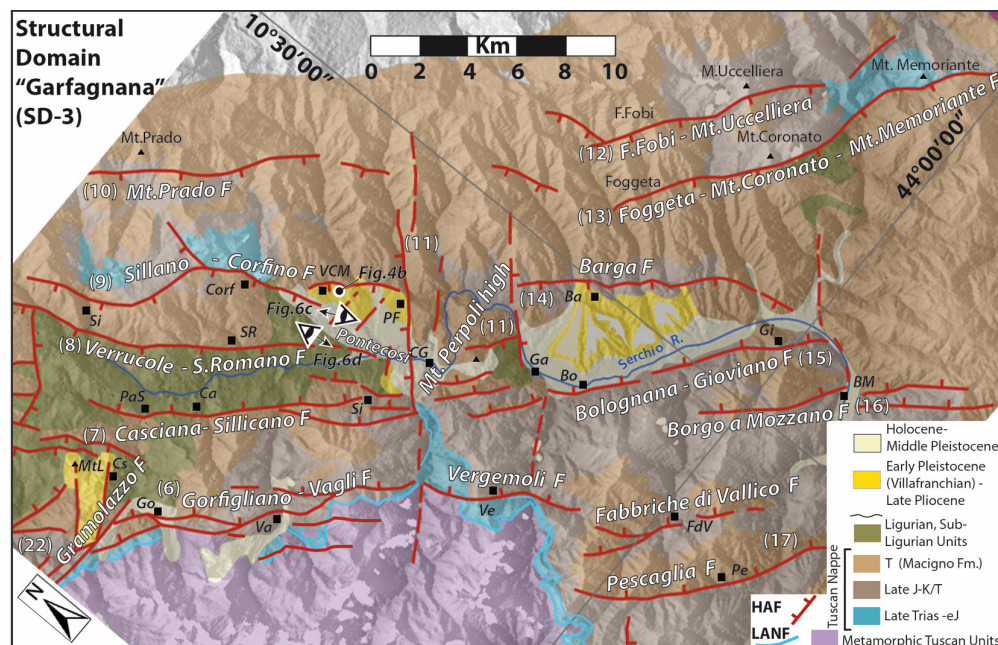
Figure 5. Main fault systems and geology in structural domain SD3 (Garfagnana). The map is derived from [56,57,77,84] and our work. Fault identification numbers are as reported in Table S1. HAF: steep normal faults; LANF: low-angle detachment faults; Ba: Barga; BM: Borgo a Mozzano; Bo: Bolognana; Ca: Casciana; CG: Castelnuovo Garfagnana; Cs: Castagnola; Corf: Corfino; Ga: Galliciano; Gi: Gioviano; Go: Gorfigliano; MtL: Mt. Lupacino; PaS: Piazza al Serchio; Pe: Pescaglia; PF: Pieve Fosciana; Si: Sillicano; SR: San Romano; Va: Vagli; VCM: Villacollemandina; Ve: Vergemoli.
