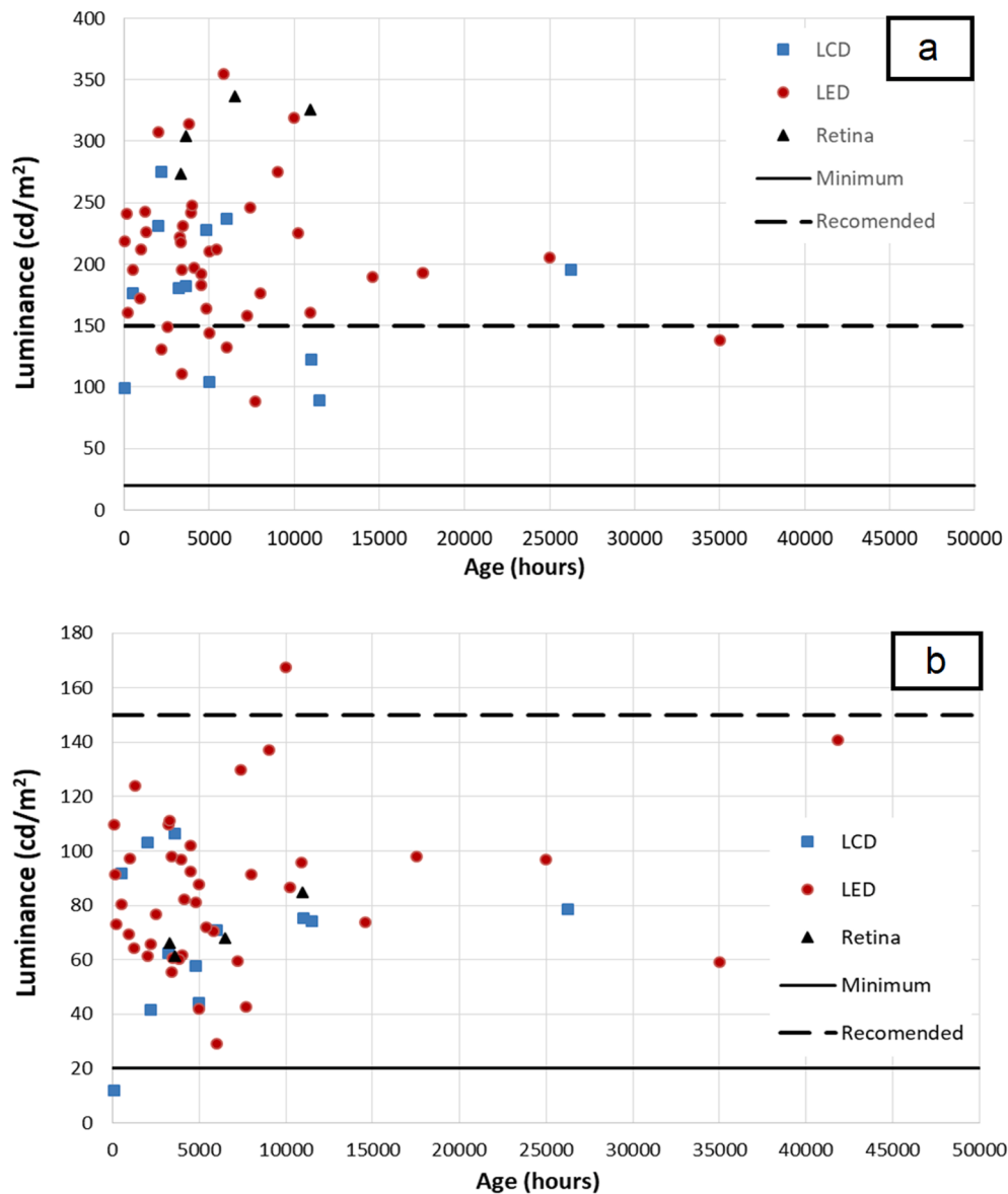
Fig. 6. Average luminance on the laptop displays in relation to the hours of use in (a) B100 configuration and (b) B50 configuration, the minimum required and recommended values indicated in [34] are shown with horizontal lines, a continuous and dotted respectively.
