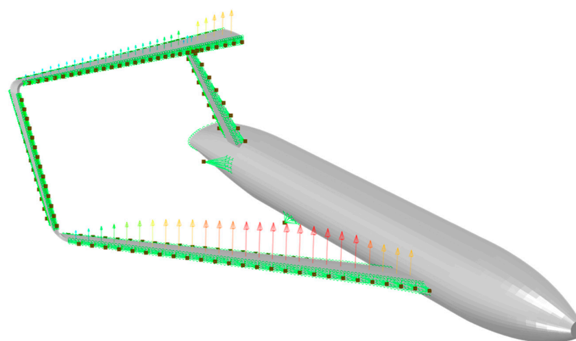
Figure 15. Secondary structures of the box-wing lifting system and aerodynamic forces (aircraft half-model).
