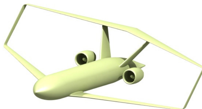
Figure 9. CAD model of the reference PrandtlPlane.
