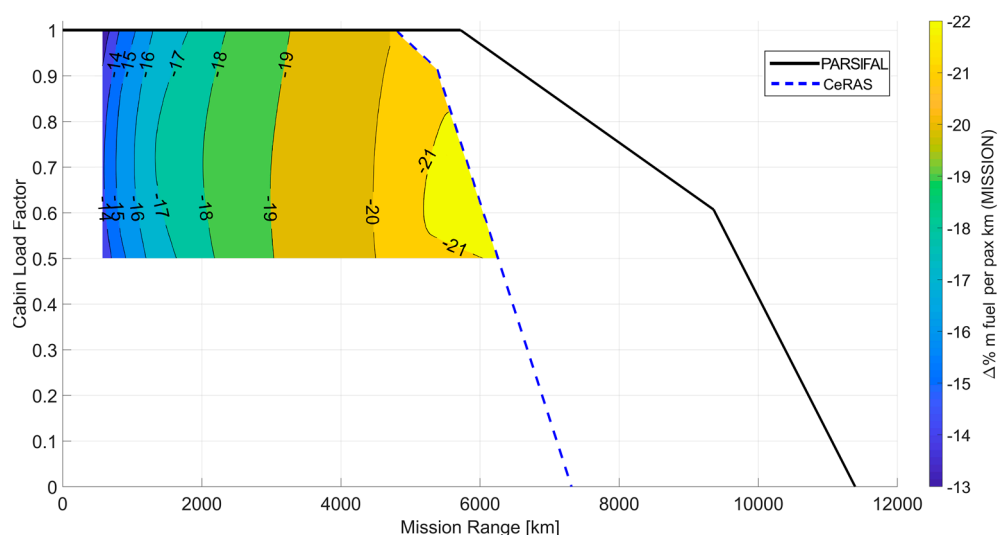
Figure 35. Comparison between the cabin load factor range diagrams (PARSIFAL PrandtlPlane vs. CeRAS CSR-01) and fuel consumption per pax km.
