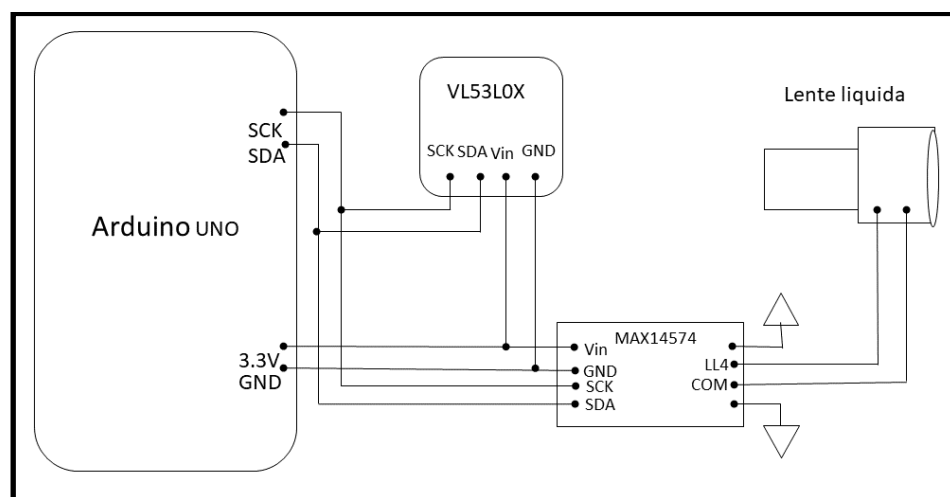
Figure 2. Autofocus system block diagram.
