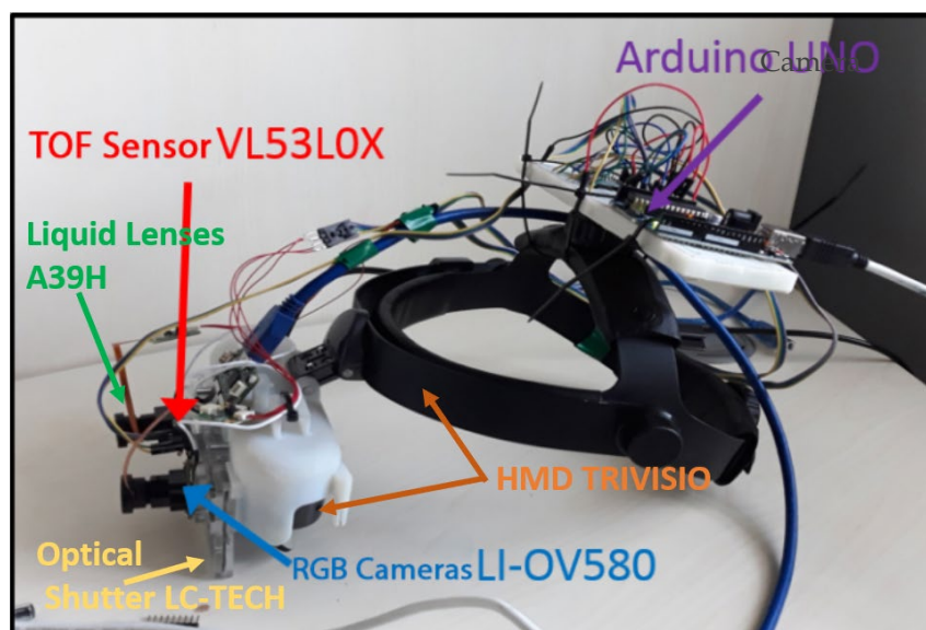
Figure 1. The Trivisio visor with the proposed autofocus system integrated.
