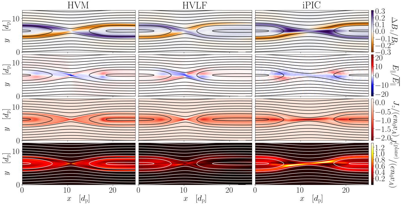
Fig. 2. Heat maps of \Delta B_z = B_z - B_z(t = 0) (first row), E_{\parallel} (second row), J_z (third row), and J_e^{(\text{in-plane})} (fourth row) for the HVM (left column, t = 237.5\Omega_p^{-1} ), HVLF (central column, t = 232.5\Omega_p^{-1} ), and iPIC (right column, t = 235.0\Omega_p^{-1} ) simulations. These times are chosen by fixing the value of the reconnected magnetic flux. This value is in the middle of the super-exponential phase. The plot is zoomed-in around the main X point. The \bar{E}_{\parallel} is the rms value of E_{\parallel} in the shown region.
