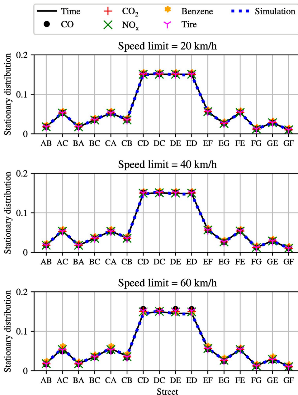
Fig 3. Distribution of emissions for the simple network with different speed limits, namely 20, 40 and 60km/h, in the entire network.
