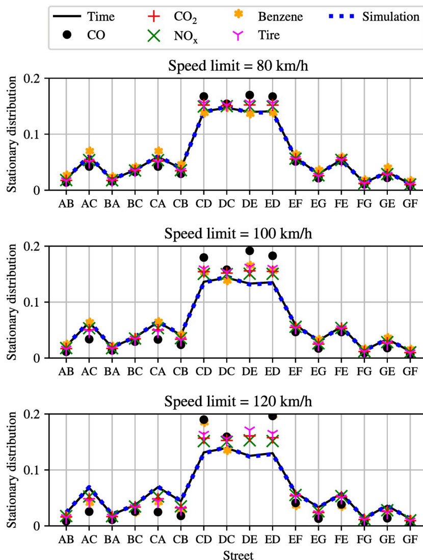
Fig 4. Distribution of emissions for the simple network with different speed limits, namely 80, 100 and 120 km/h, in the entire network.
