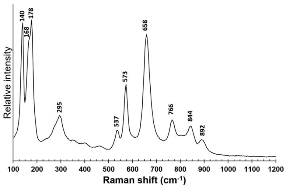
Fig. 2. Micro-Raman spectrum of bianchioniite in the range between 100 and 1200 \text{cm}^{-1} .
