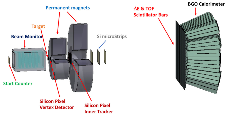
FIGURE 3 | Schematic view of the upstream region and the Magnetic Spectrometer setup.
