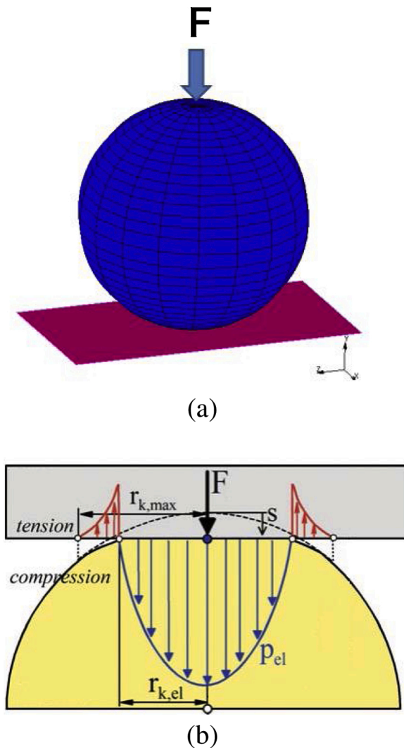
Fig. 3. a, b: a) FE model of a \text{Li}_4\text{SiO}_4 pebble; b) Characteristic pressure distribution during elastic deformation.
