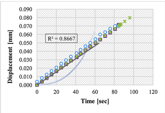
Fig. 6. Experimental vs numerical vertical displacement of pebble. The solid greys line represent the numerical data; the points indicated with circles, squares and crosses represent the experimental data. (For interpretation of the references to colour in this figure legend, the reader is referred to the web version of this article).
